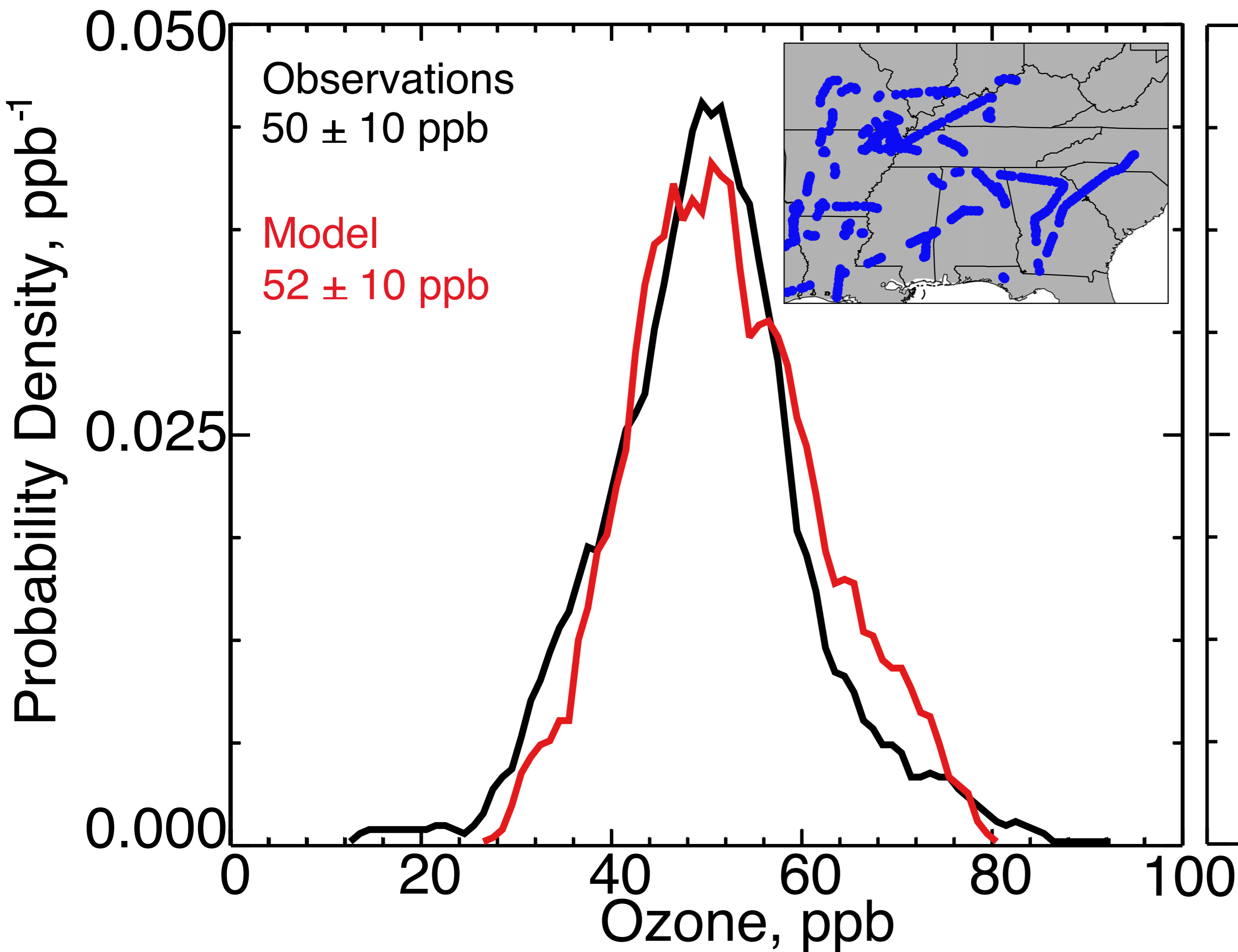
Afternoon ozone at 0.4-1.0 km altitude
