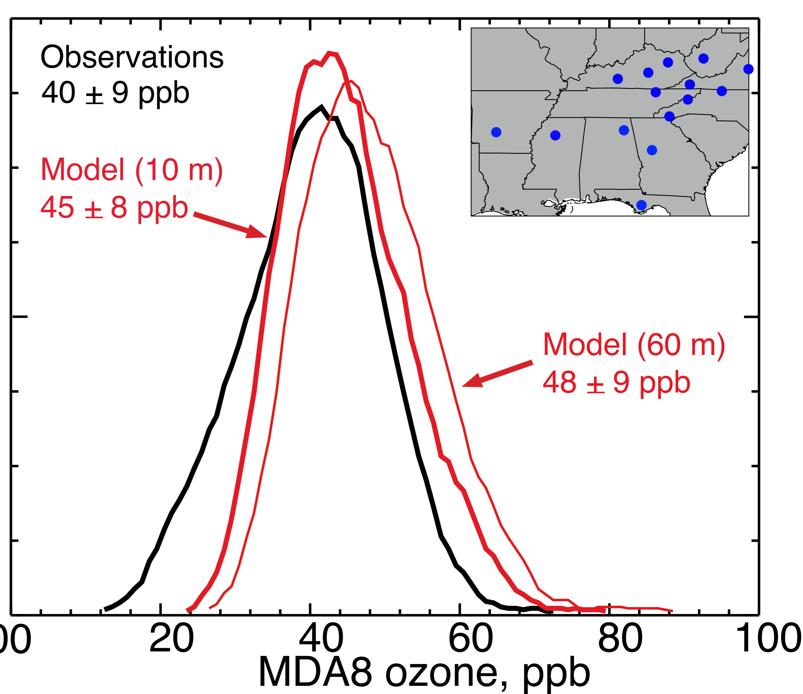
MDA8 surface ozone
