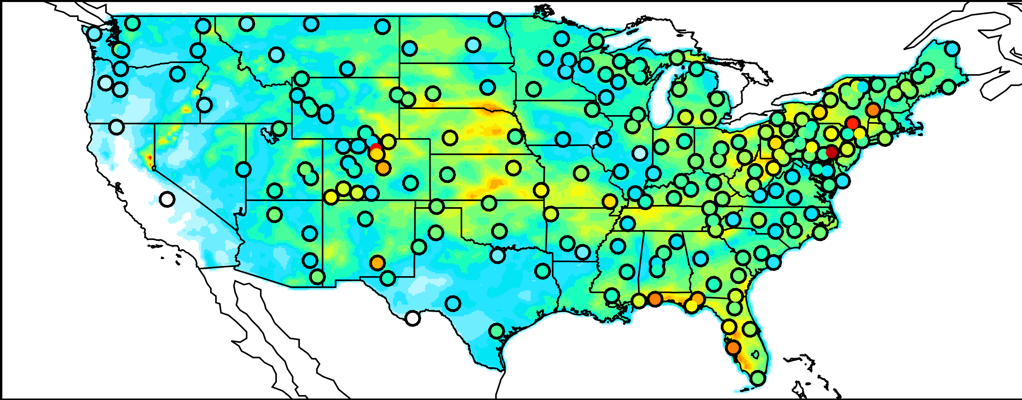
Nitrate wet deposition fluxes, Aug-Sep 2013
