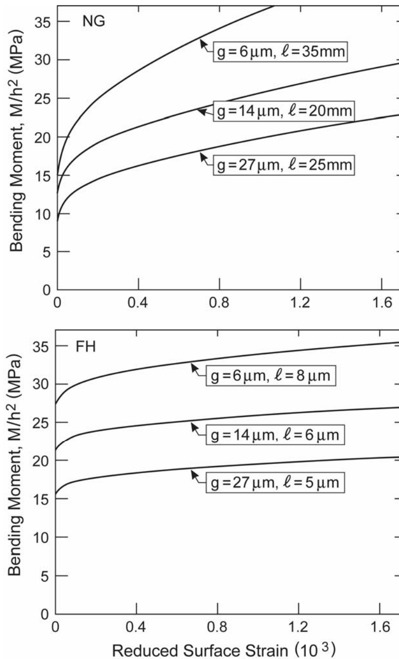
Fig. 6 Predictions of the normalized bending moment, M/h^2 , as a function of the reduced surface strain for three grain sizes all for foils having thickness h = 50 \mu\text{m} . In each case, the length parameter was chosen independently to give the best fit to the data in Fig. 1. Upper figure: NG theory and Lower figure: FH theory.
