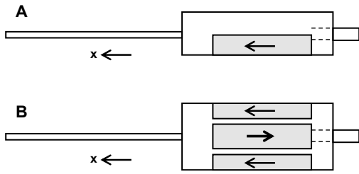
Figure 2: Top view of the MCI actuation mechanism (A) and a counterbalanced actuation mechanism (B). Actuation of the MCI generates inertial forces and torques to the user. In the counterbalanced design (B), reaction forces from the actuator and other moving components (top and bottom arrows) are cancelled by a counterweight moving in the opposite direction (middle arrow). The masses and locations of the moving components are chosen to ensure torque-free actuation.
