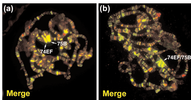
Figure 1 Colocalization of (a) Spt5 and (b) Spt6 with Pol Ilo ser2 (Pol II phosphorylated on Ser2) on Drosophila polytene chromosomes. Spt5 and Spt6 are red, Pol Ilo ser2 is green and colocalization is shown as yellow. Polytene positions 74EF and 75B are indicated. Adapted with permission from [12].
