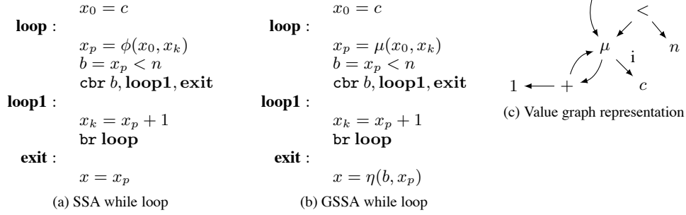
Figure 2: Representation of while loops
