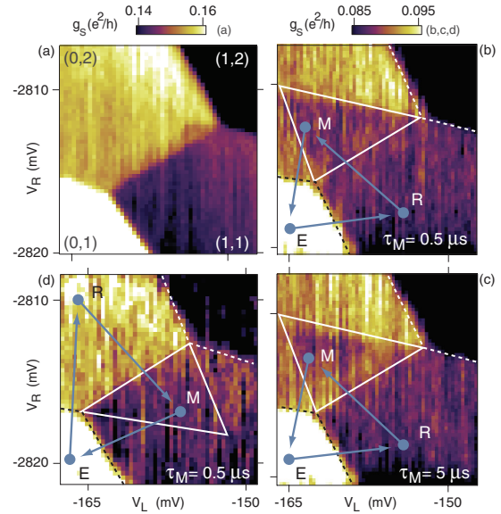
FIG. 2 (color online). Sensor conductance g_s as a function of V_R and V_L around the (1, 1) - (0, 2) transition (a) without applied pulses and (b) with the T_1 pulse cycle E \rightarrow R \rightarrow M \rightarrow E applied, \tau_M = 0.5 \mu\text{s} < T_1 . Dashed lines indicate the boundaries of (0, 1) and (1, 2) during step M . Within the pulse triangle (solid white lines), g_s is between the (1, 1) and (0, 2) values, indicating partially blocked tunneling from (1, 1) to (0, 2) , (c) with the T_1 pulse cycle, \tau_M = 5 \mu\text{s} > T_1 , and (d) the control pulse cycle, with R and M interchanged. B = 0 in each panel. Blue arrows are schematic: Point E is farther left than shown so that the pulse cycle encloses the (0, 1) - (1, 1) - (0, 2) vertex for all points M within the pulse triangle.
