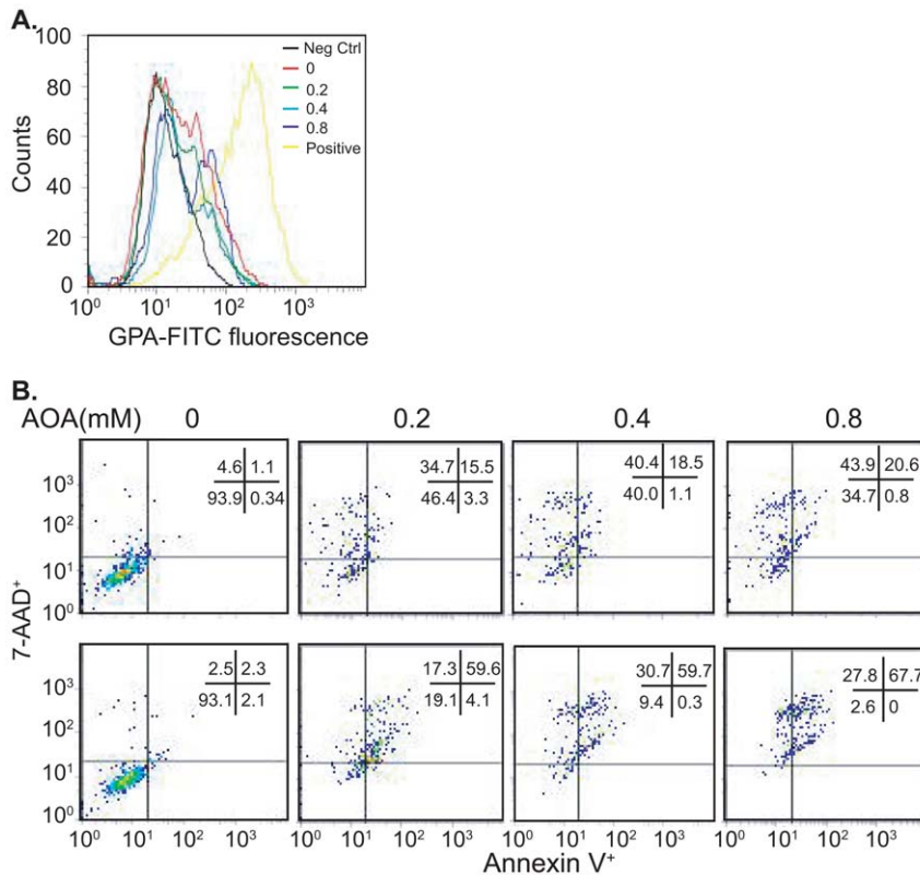
Figure 6. Supplementation by exogenous amino-oxoacetate in medium cannot induce erythroid differentiation but does induce cell death. A. Cells were treated with different concentrations of amino-oxoacetate and expression levels of the erythroid marker glycophorin A on the surface of K562 cells were assessed using a mouse FITC-conjugated anti-human glycophorin A antibody. Each histogram is representative of three experiments. B. K562 cells with or without ME2 knockdown were incubated with different concentrations of AOA for 72 h. Cell death was assessed by flow cytometry. Top: pLKO; Bottom: shME2-3. Data are representative of two independent experiments. doi:10.1371/journal.pone.0012520.g006
