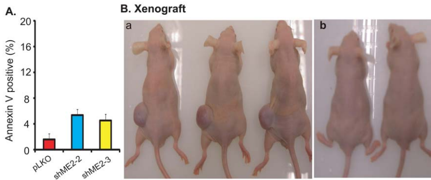
Figure 3. Stable knockdown of endogenous ME2 levels in K562 cells results in apoptosis in vitro and suppresses tumor formation from K562 cells in vivo . A: Knockdown of ME2 induces apoptosis in K562 as detected using the annexin V reagent. Data are expressed as mean \pm SD, n = 3 . B: Stable knockdown of ME2 in K562 cells failed to generate tumors in nude mice. Approximately 10^7 ME2 deficient or control K562 cells resuspended in 200 \mu l of a serum-free culture medium/Matrigel mixture (1:1) were subcutaneously implanted into female athymic nude mice as described under "Materials and Methods". Tumor-bearing mice were sacrificed after 4 weeks and the mice photographed before excision and weighing. a, Left (L): pLKO; Right (R): shME2-2; b, L and R: shME2-3. Tumors formed only in the pLKO transduced cells. doi:10.1371/journal.pone.0012520.g003
