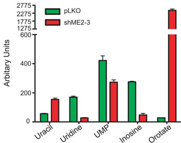
Figure 8. Knockdown of ME2 alters pyrimidine metabolism in K562 cells. The metabolites were measured by LC-MS method as described in “Materials and Methods”. doi:10.1371/journal.pone.0012520.g008
