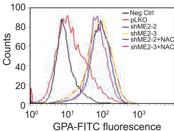
Figure 5. The antioxidant NAC cannot rescue ME2 knockdown induced erythroid differentiation in K562 cells. A: 5 mM NAC completely rescues ROS generation in K562 cells as detected by flow cytometry using CM-H 2 DCF-DA. Each histogram is representative of three experiments. B: ROS inhibition by 5.0 mM NAC did not rescue ME2 knockdown induced erythroid differentiation in K562 cells. Each histogram is representative of three experiments. doi:10.1371/journal.pone.0012520.g005
