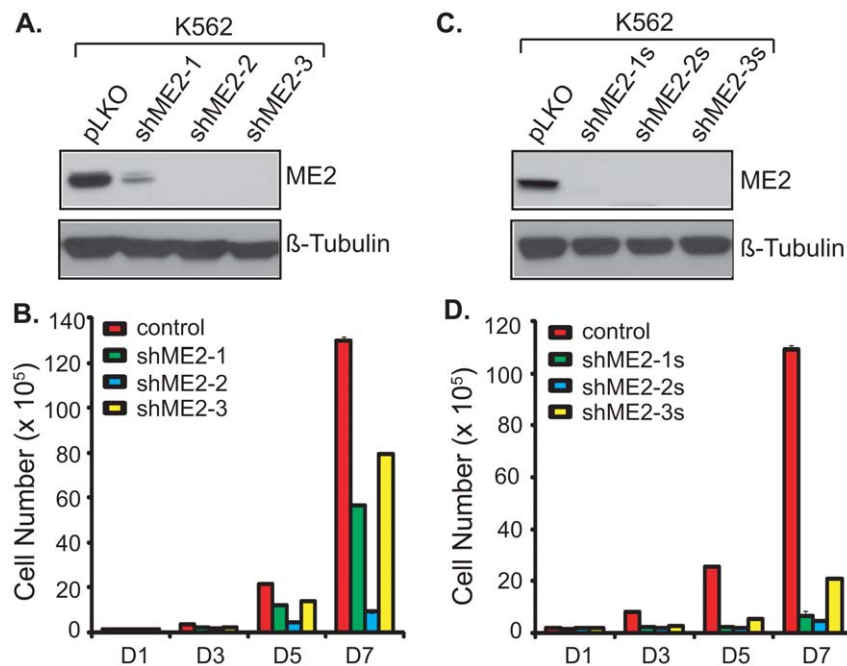
Figure 1. Effects on K562 cell proliferation of three independent shRNA hairpins targeting ME2. A: Western blot analysis using an ME2 antibody of lysate from respective pools of cells transduced with three independent ME2 shRNA lentiviruses, and following selection of puromycin for 10 days as described under "Materials and Methods". Data are representative of two independent experiments. All three pools showed marked ME2 silencing. B: Cell proliferation in K562 cells transduced with the indicated shRNA lentiviral constructs as described in "A". Data are representative of three independent experiments. C: Western blot analysis of cellular extracts in single clone K562 cells as described under "Materials and Methods" demonstrated effective knockdown of ME2 levels. Data are representative of two independent experiments. D: Cell proliferation of K562 single cell clones with ME2 knockdown derived from the corresponding pools as described in "C". Data are representative of three independent experiments. doi:10.1371/journal.pone.0012520.g001
