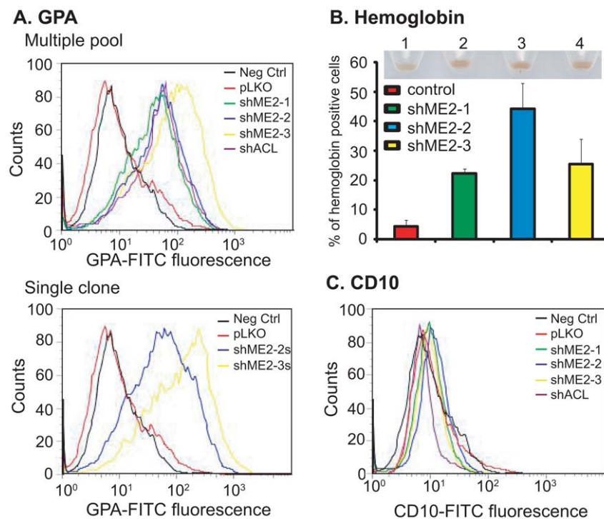
Figure 2. Stable knockdown of endogenous ME2 levels in K562 cells induces erythroid differentiation. A: Expression levels of the erythroid marker glycophorin A on the surface of control (pLKO) and ME2 knockdown cells (shME2-1, shME2-2 and shME2-3) were compared using a mouse FITC-conjugated anti-human glycophorin A antibody. As a negative control (Neg Ctrl), cells were incubated with FITC-conjugated control IgG. As a positive control, K562 cells were transduced with ATP citrate lyase (ACL) shRNA lentiviral particles (ACL inhibition is known to cause erythroid differentiation in K562 cells – referenced in the text), and incubated with mouse FITC-conjugated anti-human glycophorin A antibody. The control clone was generated by stable transduction of control pLKO vector, while clones shME2-1, shME2-2 and shME2-3 were generated using the pLKO-ME2 shRNA lentivirus. Data are representative of three independent experiments. B: The percentage of hemoglobin-expressing cells in control (pLKO) and ME2 knockdown (shME2-1, shME2-2 and shME2-3) cell populations was determined by benzedrine staining. Plotted is the mean \pm SD from triplicate samples from a representative experiment. Insert: cell pellets from ME2 knockdown cells. 1: pLKO; 2: shME2-1; 3: shME2-2; 4: shME2-3. Increased brown color is clearly visible in lanes 2, 3 and 4. C: Expression levels of the megakaryocytic marker CD10 on the surface of control (pLKO) and ME2 knockdown cells (shME2-1, shME2-2 and shME2-3) were compared using a mouse FITC-conjugated anti-human CD10 antibody. As a negative control (Neg Ctrl), cells were incubated with FITC-conjugated control IgG. The control clone was generated by stable transduction of control pLKO vector, while clones shME2-1, shME2-2 and shME2-3 were generated using the pLKO-ME2 shRNA let virus. Data are representative of three independent experiments.
