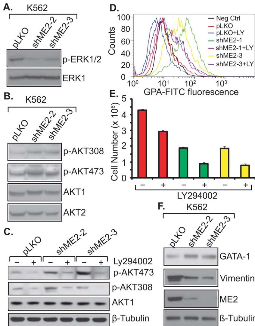
Figure 7. Effects of ME2 knockdown on signaling pathways, and GATA-1 and vimentin expression. K562 cells with or without ME2 knockdown were lysed with RIPA lysis buffer (50 mM Tris-HCl, pH 8.0, 150 mM NaCl, 1% Triton X-100, 1 mM EGTA) containing 1 mM PMSF and a protease inhibitor cocktail and subjected to centrifugation at 15,000 \times g for 10 min at 4^\circ\text{C} to remove debris. After lysis, equal aliquots of protein lysate were resolved by Western blotting. Western blots were probed with anti-phospho-ERK1/2, anti-ERK1, anti-p-AKT308, anti-AKT472, anti-AKT1/2, anti-GATA-1, anti-vimentin and anti- \beta -tubulin. A, phospho-ERK1/2 activity in ME2 knockdown K562 cells. B, Phospho-AKT detection in ME2 knockdown K562 cells. C, 10 \mu\text{M} PI3K inhibitor, LY294002, inhibits p-AKT activity. D, LY294002 rescue of differentiation in ME2 knockdown K562 cells. E, The effect of LY294002 on the proliferation of K562 cells with or without ME2 knockdown. F, The expression difference of GATA-1 and vimentin in ME2 knockdown cells. Data are representative of three independent experiments. doi:10.1371/journal.pone.0012520.g007
