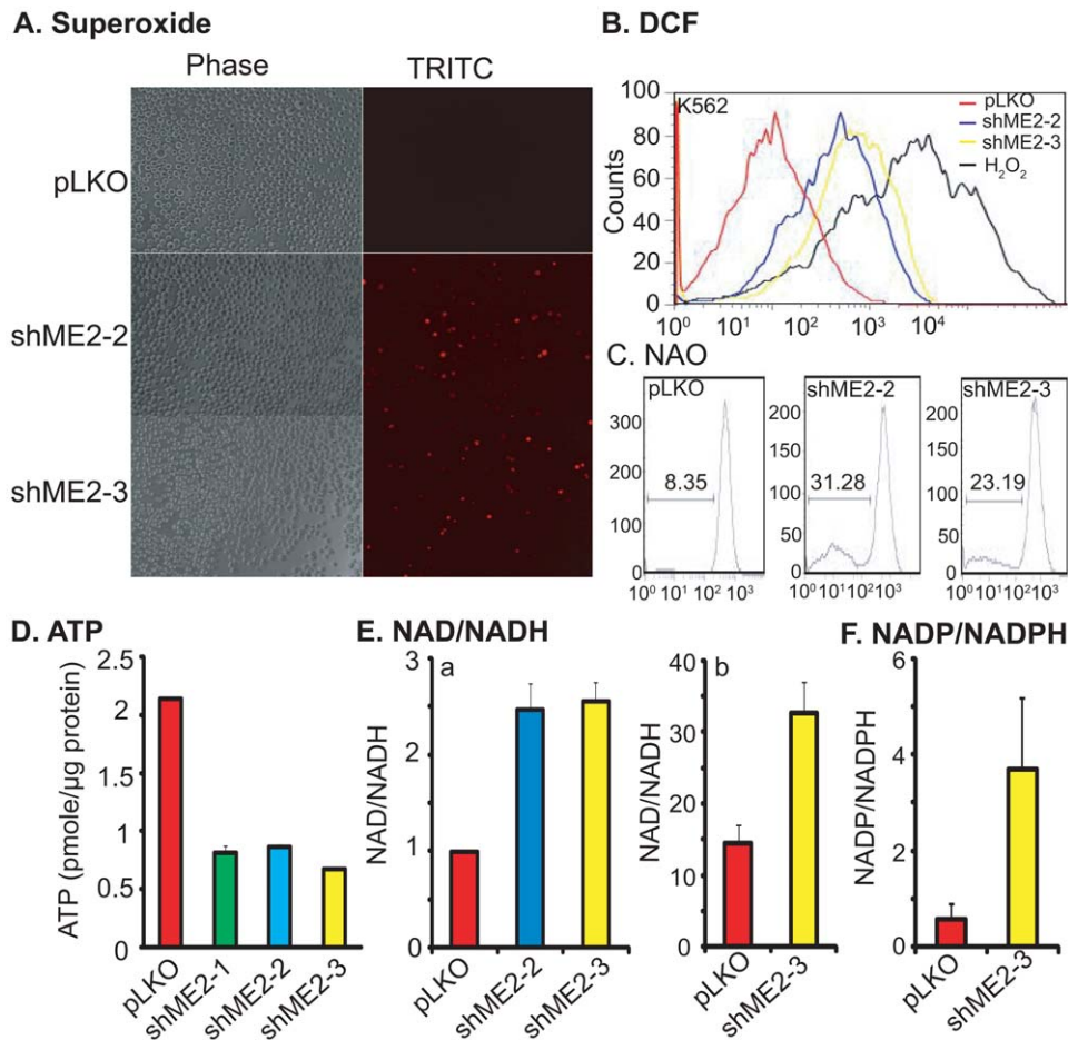
Figure 4. Depletion of endogenous ME2 enhances ROS generation, increases NAD + /NADH and NADP/NADPH ratios and decreases ATP levels. A: Accumulation of mitochondrially generated superoxide in K562 ME2 knockdown cells as detected by MitoSOX. Data are representative of two independent experiments. B: Increased ROS in K562 ME2 knockdown cells detected by flow cytometry using CM-H 2 DCF-DA. Each histogram is representative of three experiments. C: Comparison of oxidative damage to cardiolipin in ME2 knockdown versus control K562 cells. M1 indicates subpopulation of cells that lost NAO signal due to cardiolipin oxidation. D: Depletion of ME2 inhibits ATP production in K562 cells. Data are expressed as mean \pm SD, n = 3. E: Depletion of ME2 increases NAD + /NADH ratio. a, NAD + and NADH were measured by NAD/NADH Assay Kit (Abcam, San Francisco, CA) as described in "Materials and Methods". Data are expressed as mean \pm SD, n = 3. b, NAD + and NADH were measured by LC-MS methods as described in "Materials and Methods". F: Depletion of ME2 increases NADP/NADPH ratio in ME2 knockdown cells. NADP and NADPH were measured by LC-MS methods as described in "Materials and Methods". doi:10.1371/journal.pone.0012520.g004
