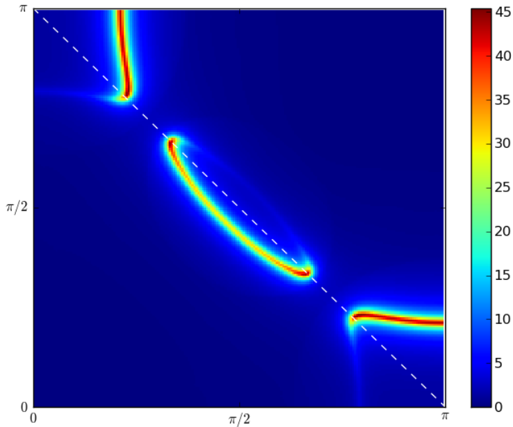
FIG. 7. Electron spectrum function at zero frequency as a convolution of z_\alpha and the \psi_\pm fermions. In the plot we chose the following parameters: \varrho = 0.1t , T = 0.2t and the SDW gap \lambda = 0.2t . The white dashed line shows the boundary of the diamond magnetic Brillouin zone of the commensurate (\pi, \pi) AFM order.
