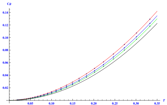
FIG. 4: Plot of nodal fermion contribution to specific heat with v_\Delta/v_{f0} = 1/5 , v_\Delta/v_{f0} = 1/10 , v_\Delta/v_{f0} = 1/20 from the top to bottom. The horizontal axis is in scale of T/T_c . The curves are y = x^{1.86} (red), y = x^{1.91} (blue), y = x^{1.945} (green), y = x^2 (black).
