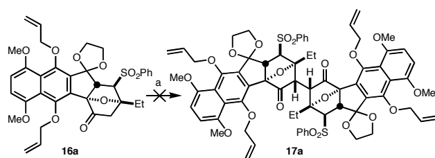
Scheme 4. Attempted oxidative dimerization of 16a . Reagents and conditions: a) LHMDS, HMPA, THF, -78 °C, 2 h; then Cp 2 FePF 6 , -60 °C, 72 h, 0%. LHMDS = lithium bis(trimethylsilyl)amide, HMPA = hexamethylphosphoramide, Cp 2 FePF 6 = ferrocenium hexafluorophosphate.
