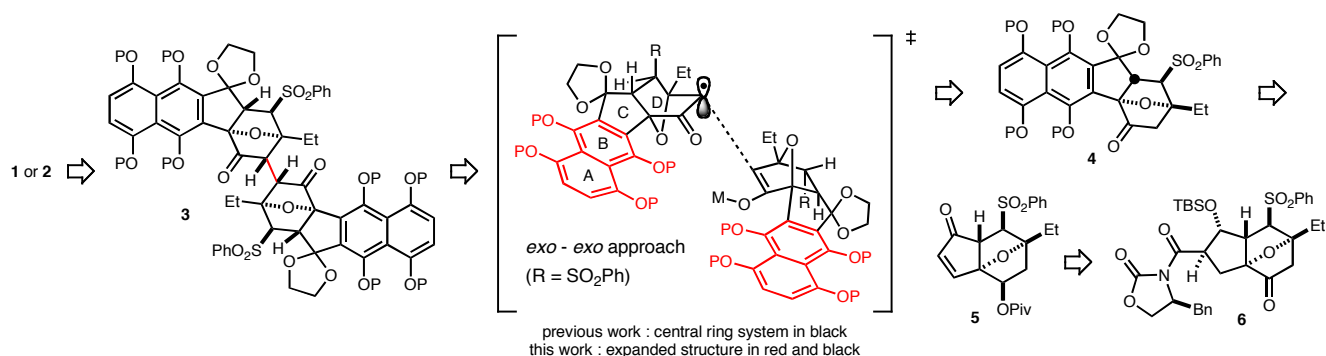
Scheme 1. Synthesis plan.
