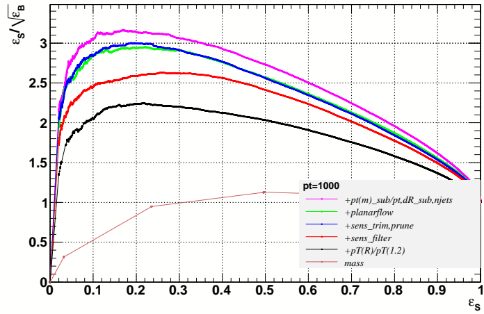
FIG. 14: Significance gain from the multivariate analysis for p_T^{\text{jet}} = 200, 500, 1000 GeV.
