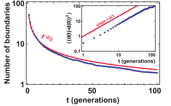
FIG. 6 (Color online) The number of monoallelic domain boundaries as a function of time in the undulating-front model. The simulation of 100 demes averaged over 100 runs is plotted in blue (dots), and the theoretically expected decay of the number of boundaries as t^{-2/3} [see Saito and Müller-Krumbhaar (1995)] is plotted in red (solid line). Note that the agreement between the theory and the simulations is not expected during the transitory regime at early times. At t = 0 , each site is assigned either allele one or allele two with equal probability. Inset: Log-log plot of the mean square displacement of the domain boundaries as a function of time in the same set of simulations as the main plot. The blue dots are the simulation data, and the solid red line is the expected slope according to Saito and Müller-Krumbhaar (1995).
