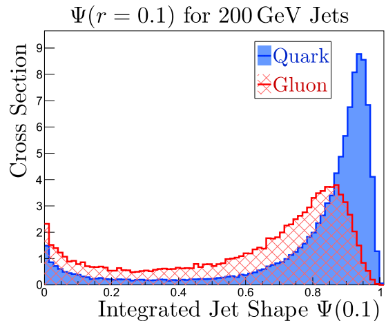
FIG. 1: Data on the integrated jet shape \Psi(r) is usually published only when averaged over all events. Here we show the distribution of \Psi(0.1) , for quarks (blue, solid) and gluons (red, hollow). The event-by-event distributions of \Psi(r) and other observables are much more important for gluon tagging than average values.
