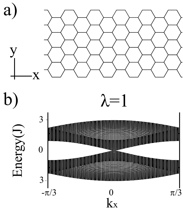
FIG. 5: a) The strip geometry considered in the text, with finite extent in the y direction, and armchair edges running parallel to x . b) Spectrum of the (static) armchair ribbon shown in panel a) with a width of 100 lattice sites in the y direction. Energy is plotted in units of J .
