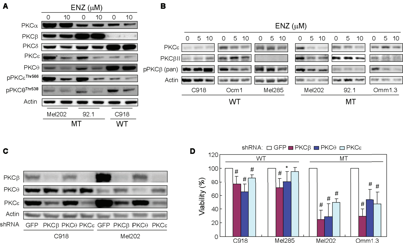
Figure 8. PKCβ, PKCε and PKCθ are functionally important for UM cells harboring GNAQ mutations. A and B, enzastaurin reduced the expression and phosphorylation of PKCβ, PKCε and PKCθ. Cells were treated with enzastaurin for 6 hours in the absence of serum (A) or for 72 hours in the presence of 10% FBS (B). pPKCε Thr566 was detected using pan p-PKC antibody raised against pPKCε Thr410. Note that the expression of PKCβ was under detectable level of Western blot in Mel285 cells (B). C, knockdown of PKCβ, PKCε, and PKCθ by shRNA. C918 and Mel202 cells were infected with lentiviruses expressing shRNA for each PKC isoform for 4 days and protein levels of these isoforms were determined by immunoblot blot analysis. D, Effects of knockdown of PKCβ, PKCε, and PKCθ on viability of UM cells. Cell viability was determined 4 days after infection with lentivirus expressing PKC shRNA using MTS assay. Results are presented as mean ± SD of percent viability from 3 independent experiments. *P<0.05 and # P<0.01, versus cells expressing GFP control shRNA. doi:10.1371/journal.pone.0029622.g008
