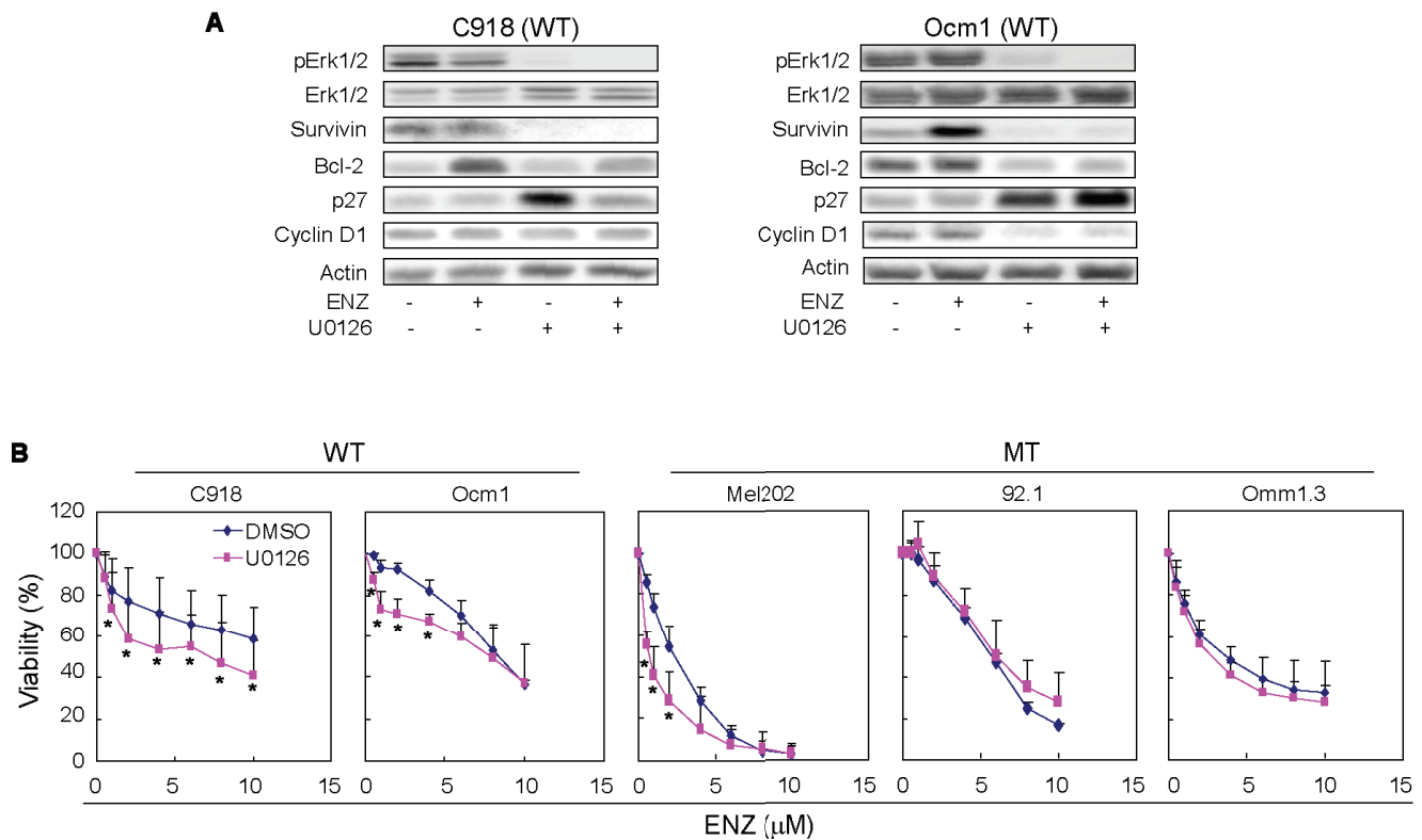
Figure 7. Effect of MEK inhibition on the antiproliferative action of enzastaurin. A, expression of Erk1/2, phospho-Erk1/2, survivin, Bcl-2, cyclin D1, and p27 Kip1 in C918 and Ocm1 cells treated with enzastaurin in the absence or presence of U0126 (20 μM) for 72 hours. B, effect of U0126 on the antiproliferative activity of enzastaurin. Assay was performed as described in Figure 1 in the absence or presence of 10 μM U0126. Results are presented as mean ± SD of percent viability from 4–5 independent experiments. * P < 0.05, versus DMSO at the same dose of enzastaurin. doi:10.1371/journal.pone.0029622.g007
