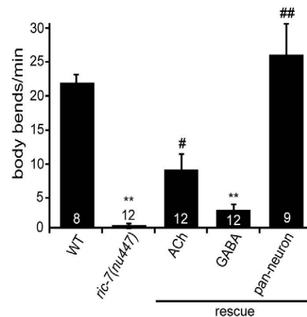
Figure 1. Aldicarb response and locomotion defects in ric-7 mutants. (A) A schematic illustrating the ric-7 gene structure is shown. Deleted regions (bar), point mutations (arrows), and the site utilized for GFP/mCherry tagging are indicated. (B–C) Aldicarb-induced paralysis (B) and locomotion rate (C) are compared for the indicated genotypes. The number of trials (~20 animals/trial, B) or the number of animals analyzed (C) are indicated for each genotype. For rescue experiments, ric-7 transgenes are indicated as follows: ACh ( unc-17 promoter), GABA ( unc-25 promoter), pan-neuron ( snb-1 promoter), muscle ( myo-3 promoter). Values that differ significantly from wild type (**, p < 0.001 , Student's t-test) and from ric-7 mutants (#, p < 0.01 ; ##, p < 0.001 , Student's t-test) are indicated. Error bars indicate SEM. doi:10.1371/journal.pgen.1002464.g001
