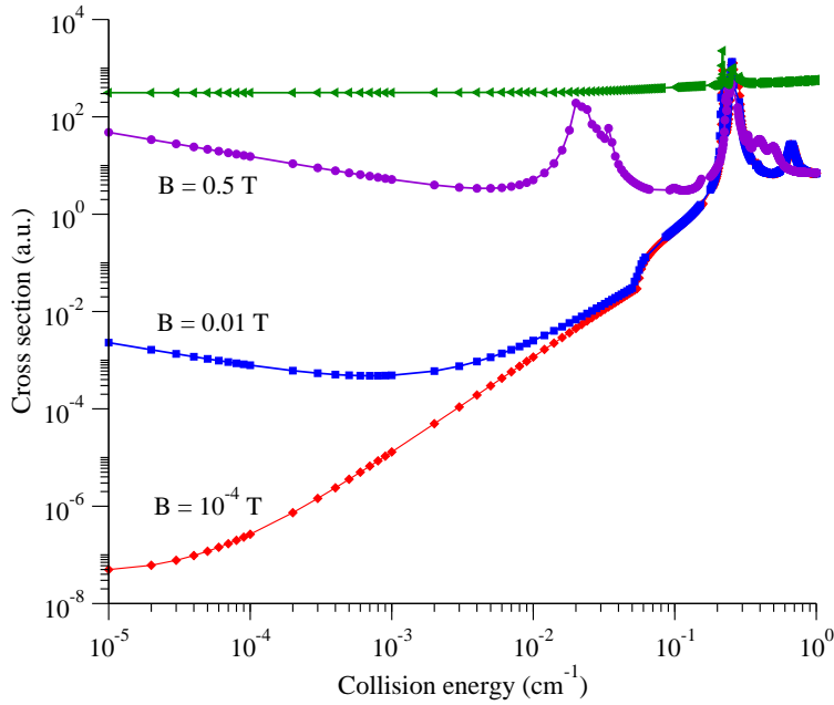
Figure 2: Cross sections for elastic scattering and spin relaxation in {}^3\text{He}\text{--OH} collisions as functions of collision energy at different magnetic fields indicated in the graph. The elastic cross section is shown for B = 10^{-4} T.
