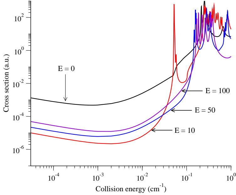
Figure 3: Cross sections for elastic scattering and spin relaxation in ^3\text{He}\text{-OH} collisions as functions of collision energy calculated for several electric field strengths (in kV/cm) indicated in the graph. The magnetic field is fixed at 0.01 T.
