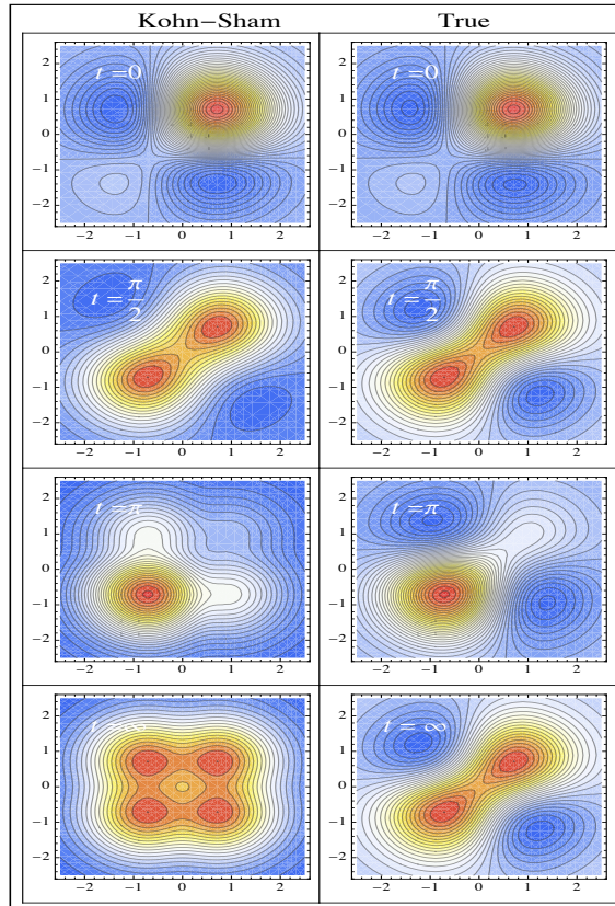
Figure 5.8: Time evolution of the real part of the Kohn-Sham density matrix \Re\rho_{ks}(x, x', t) (left column) and true OQS density matrix \Re\rho_{open}(x, x', t) (right column) for the pure dephasing master equation.
