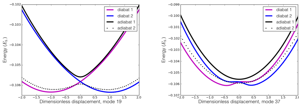
Figure 7.4: Energies of adiabatic, and quasidiabatic transfer states as a function of dimensionless displacement along [2,2'] dithia-anthracenophane’s 19^{th} (left), and 37^{th} (right) normal mode. In the figure on the left it’s immediately clear by inspection that the diabatic states are more harmonic than the adiabatic states. The figure on the right is an example where the accuracy of using Eq. ( 7.10) is questionable.
