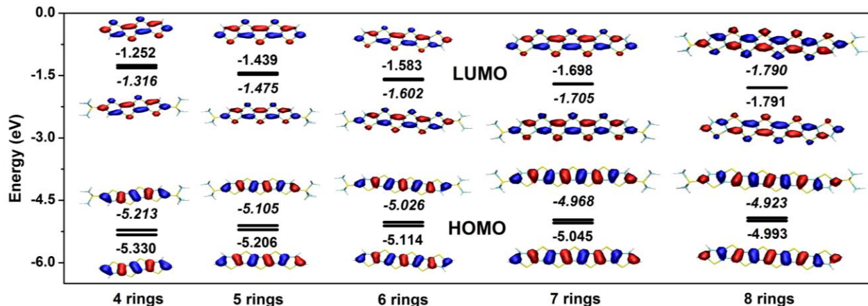
Figure 4. DFT/B3LYP/6-31G** energy levels around the HOMO-LUMO gap region and molecular orbital topologies of the HOMO and LUMO of tetra(penta, hexa, hepta, and octa)thienoacene and TMS-T4(5, 6, 7, and 8)-TMS. The italicized energy values correspond to those of the TMS-T n -TMS oligomers.
