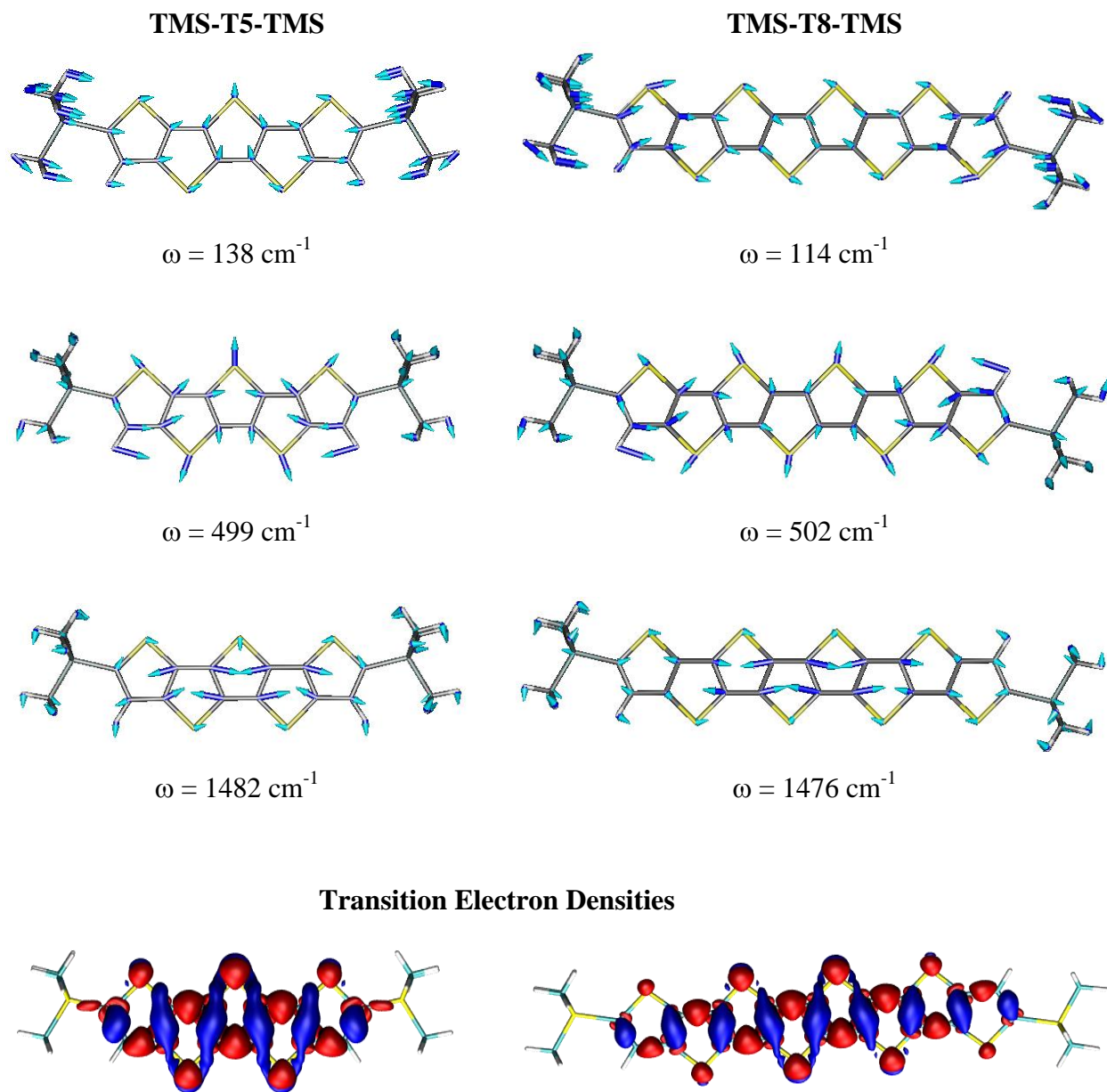
Figure 5. (top) Illustrations of the normal modes yielding the largest Huang-Rhys factors and (bottom) electron density change in the S 0 -S 1 electronic transition of TMS-T5-TMS and TMS-T8-TMS (left and right, respectively). The low-frequency modes involve mostly the sulfur atoms, whereas the high-frequency modes involve the carbon atoms.
