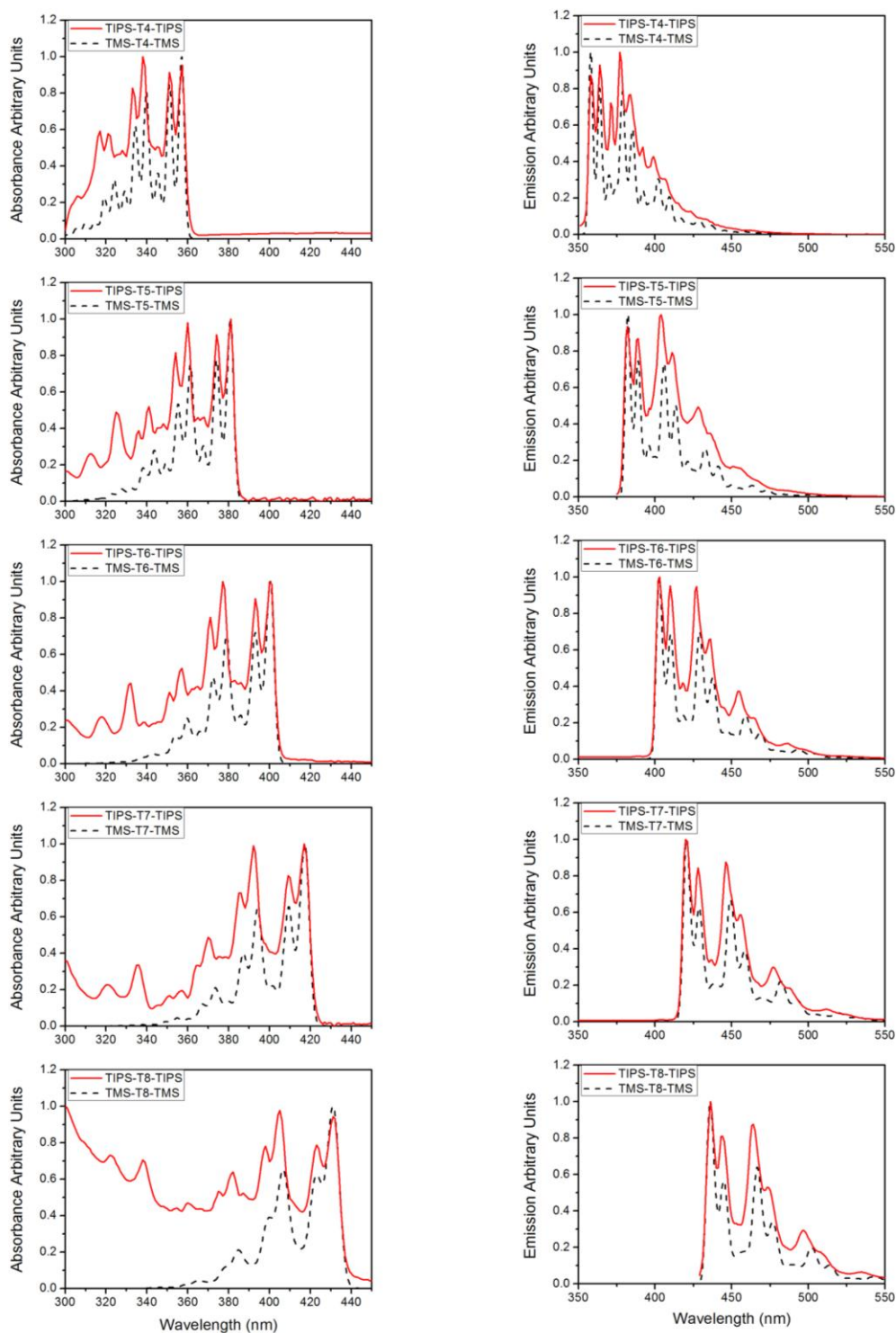
Figure 7. Normalized UV-Vis absorption and fluorescence experimental-spectra of TIPS- T_n -TIPS (solid lines). The dashed lines represent the simulated (theoretical) spectra convoluted with Gaussian functions. Note that for computational efficiency, in all theoretical simulations we used TMS substituents instead of TIPS substituents. The onset of the simulated spectra is chosen to correspond to experimental onset.
