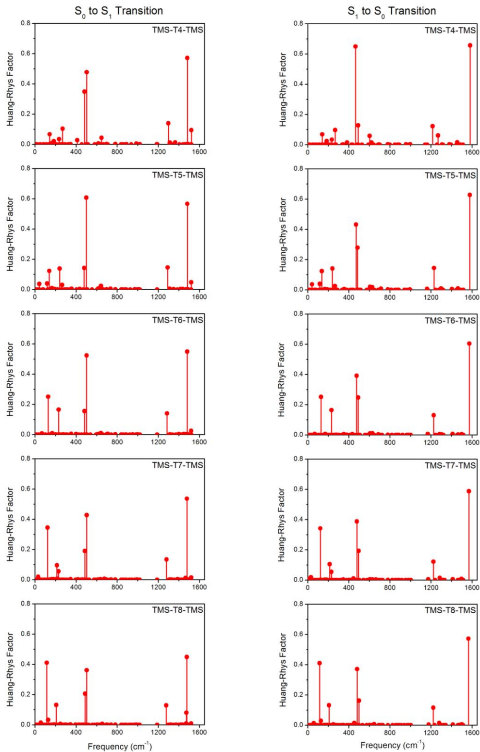
Figure 6. DFT/TD-DFT/B3LYP/6-31G** Huang-Rhys factors related to the S_0 \rightarrow S_1 and S_1 \rightarrow S_0 transitions of TMS- T_n -TMS as a function of the normal-mode frequency.
