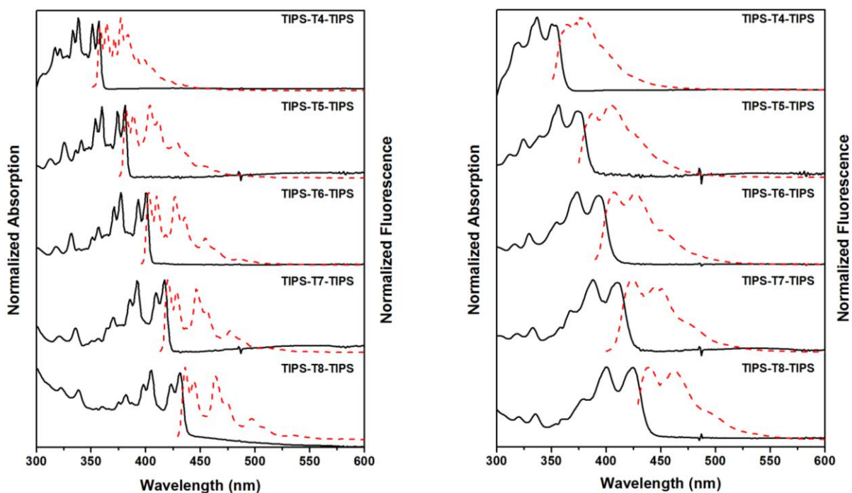
Figure 3. Normalized UV-Vis absorption (solid lines) and fluorescence emission (dashed lines) spectra of TIPS- T n -TIPS oligothiophenes in MeTHF recorded at 78 K (left) and at room temperature (right).
