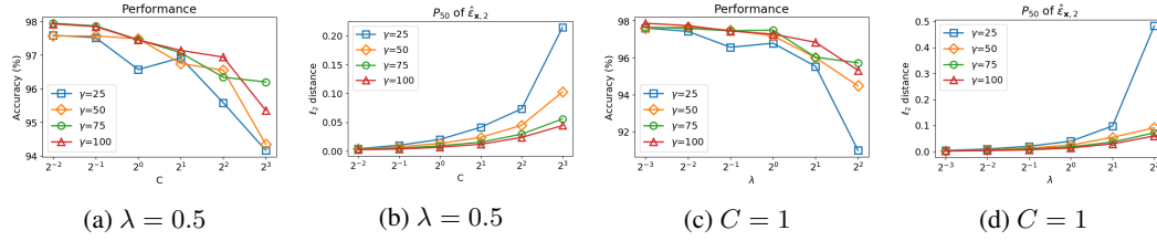
Figure 2: Parameter analysis on MNIST dataset. P_{50} of \hat{\epsilon}_{x,2} is the median of \hat{\epsilon}_{x,2} in the testing data.
