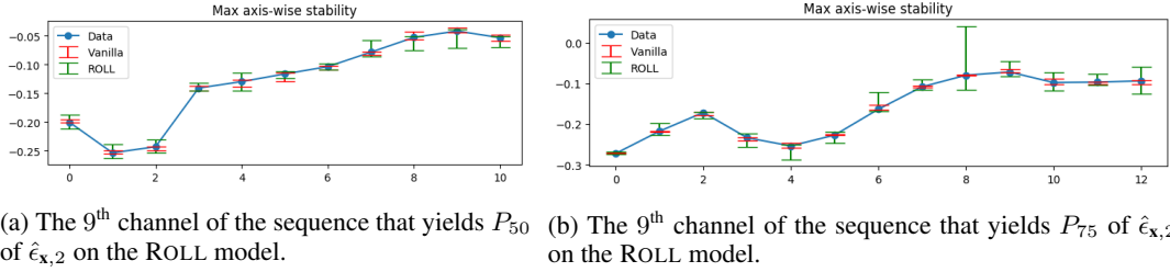
Figure 3: Stability bounds on derivatives on the Japanese Vowel dataset.
