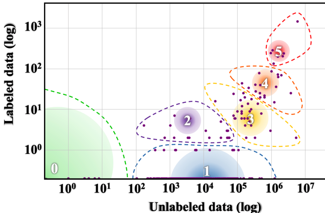
Figure 1.1: Resource Distribution by Language Type (Joshi et al., 2020)
