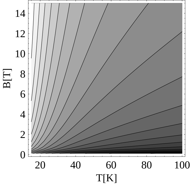
FIG. 3: Contour plot (with logarithmic spacing) of the thermoelectric conductivity \alpha_{xy} (Eq. 2.3) as a function of temperature T and magnetic field B , for parameters \hbar v = 47 meV \text{\AA} , \delta - \delta_I = 0.025 and \tau_{\text{imp}} = 10^{-12} s estimated for LSCO. In the ordered low temperature regime T < T_c \approx 30 K, Eq. (2.3) will receive modifications.
