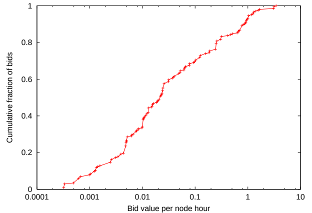
Figure 5: Cumulative distribution of bid values per node hour.
