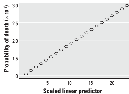
Figure 4. Cumulative normal curve versus a standardized predictor (the sum of the effects of all risk factors) over the range of exposures that correspond to daily death rates of between 1 and 3 per million, which is the observed range of variation in U.S. cities. It is quite linear in the predictor.
