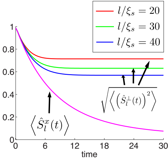
FIG. 8: The dynamics of the average value of the magnitude of spins, \sqrt{\langle (\hat{S}_l^\perp(t))^2 \rangle} , and the average of the x component of spins \langle \hat{S}_l^x(t) \rangle . Here y axis is scaled such that the initial values take the maximum value of 1. Here we took L/\xi_s = 200 , K_s = 20 and the integration lengths l/\xi_s = 20, 30, 40 . The magnitude of spins decays only due to the spin waves with wavelengths shorter than the integration length l , and the decay of the magnitude stops around the time scale of \sim \frac{l}{4c_s} . On the other hand, all spin waves contribute to the evolution of the x component of magnetization, which keeps decaying [68].
