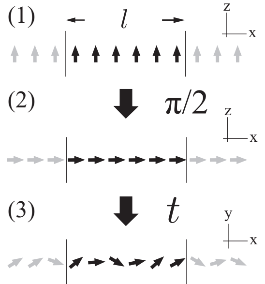
FIG. 1: Ramsey sequence for one dimensional system with two component bosons considered in this paper. (1) All atoms are prepared in spin up state; (2) \pi/2 pulse is applied to rotate each atom into the x direction; (3) spins freely evolve for time t . In actual experiments, final \pi/2 pulse is applied to measure the x component of spin. The imaging step (4) is omitted in the illustration. In this paper, spin operators refer to the ones before the final \pi/2 pulse.
