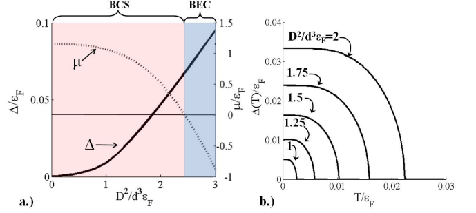
FIG. 4. (color online) Numerical solutions of the BCS gap equation (7) for the nearest-neighboring layer dipole potential (6), at fixed particle density, and with d/\lambda_F = 1 , where \lambda_F = 2\pi/k_F is the Fermi wavelength. (a) T = 0 BCS pairing as a function of interaction strength D^2/d^3 (where energies are measured with respect to the Fermi energy \epsilon_F of the unpaired system). Solid line shows solution for \Delta , and dotted line shows chemical potential \mu . The BCS regime ( \mu > 0 ) and BEC regime ( \mu < 0 ) are highlighted in red and blue respectively. (b) Temperature profile of the BCS gap for interaction strengths: D^2/d^3\epsilon_F = 2, 1.75, 1.5, 1.25 , and 1 (highest to lowest respectively).
