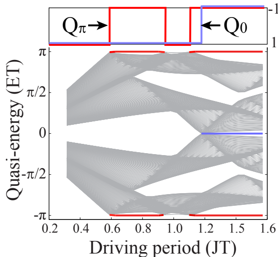
FIG. 3: (Color online.) Floquet MFs with two distinct flavors. Quasi-energy spectrum of H_{eff} and topological charges ( Q_0 and Q_\pi ) are plotted for varying period T of the drive. Since the quasi-energy is defined up to an integer multiple of 2\pi/T , it can support Floquet MFs at E = \pi/T (thick red line) as well as E = 0 (thick blue line). The appearance of the two MF flavors is not necessarily correlated, and a single Floquet MF is present in much of the parameter space. The parameters are \mu_1 = -J , \mu_2 = -3J , B = J , \Delta = 2J , and 2ka = \pi/4 .
