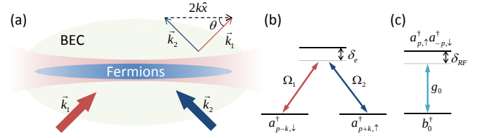
FIG. 1: (Color online.) (a) Optically trapped fermionic atoms form a 1D quantum wire inside a 3D molecular BEC. Two Raman beams propagate along \vec{k}_1 and \vec{k}_2 directions, respectively. The recoil momentum \vec{k}_1 - \vec{k}_2 = 2k\hat{x} is parallel to the quantum wire. (b) Raman coupling between two fermionic states a_{\uparrow} and a_{\downarrow} induces a 2k momentum change from photon recoil. (c) RF-induced atom-molecular conversion.
