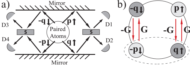
FIG. 1: Illustrations of using two-atom interference to measure the relative phase between different components of molecules after dissociation. a) Scheme I: Free propagating atoms are reflected in mirrors and mixed in beam splitters denoted by S. Coincidences are counted between detectors on opposite sides, e.g. D 1 and D 3 . b) Bragg pulses with wave-vectors \mathbf{G} = \mathbf{p} - \mathbf{q} and -\mathbf{G} are used to exchange (atomic mirrors) or mix (atomic beam-splitters, S) components \mathbf{q} \uparrow and \mathbf{p} \uparrow , as well as -\mathbf{q} \downarrow and -\mathbf{p} \downarrow ( |\mathbf{q}| = |\mathbf{p}| ). In scheme II, the Bragg pulse applied at the beginning of expansion carries out reflections on mirrors and mixings in beam splitters in a single operation.
