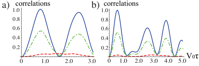
FIG. 3: Integrated noise correlations \langle \delta N_{V_\uparrow} \delta N_{V_\downarrow} \rangle as a function of V_0\tau a) for a Bragg pulse amplitude V_0/E_R = 2 , and b) for a Bragg pulse amplitude V_0/E_R = 20 . Blue, Green(dash-dotted line) and Red(dashed line) curves correspond to \Delta\phi = \phi_{\mathbf{k}} - \phi_{\mathbf{k}-\mathbf{Q}} = 0, \pi/2 and \pi , respectively.
