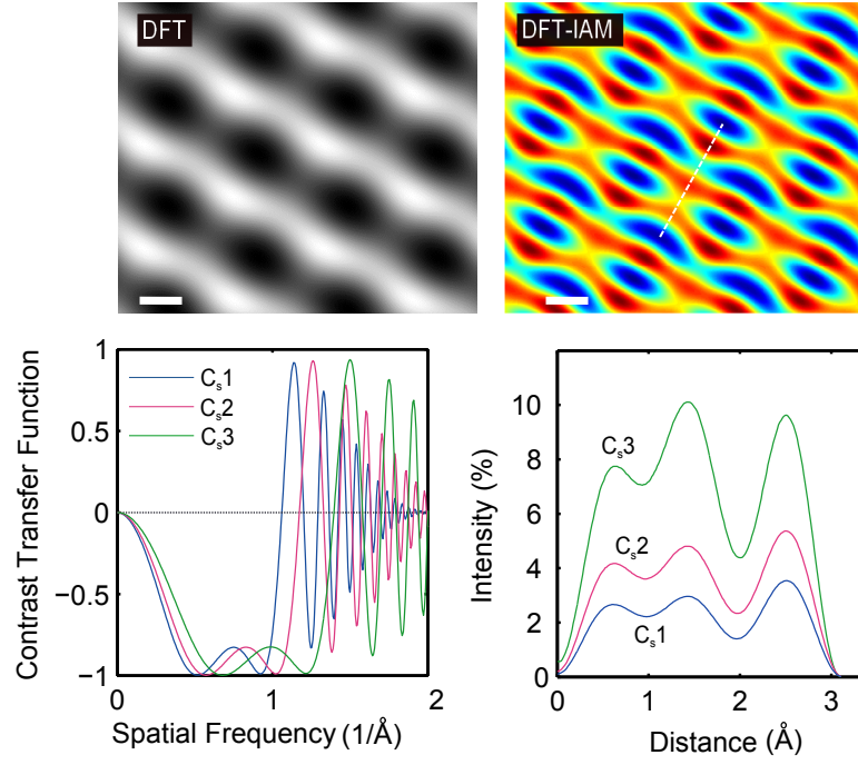
FIG. 2: Calculations of total potential based on first-principles.
