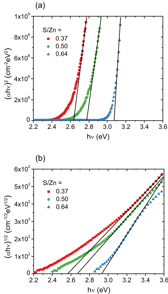
FIG. 4. Determination of the optical band gaps of various compositions of Zn(O,S) by treating the films as (a) nanocrystalline and (b) amorphous. (a) Plot of (\alpha h\nu)^2 versus h\nu yields E_g = 2.63, 2.78 , and 3.08 for Zn(O,S) with S/Zn ratios of 0.37, 0.50, and 0.64, respectively. (b) Plot of (\alpha h\nu)^{1/2} versus h\nu gives E_g = 2.57, 2.68 , and 2.92 for Zn(O,S) with S/Zn ratios of 0.37, 0.50, and 0.64, respectively.
