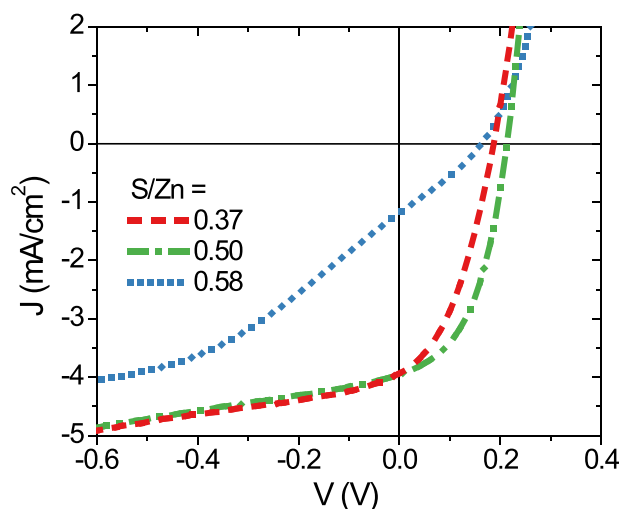
FIG. 1. Current density-voltage characteristics of Mo/SnS/Zn(O,S)/ZnO/ITO thin film solar cells with various compositions of Zn(O,S) under microscope lamp illumination ( \sim 10 \text{ mW/cm}^2 ). Reprinted with permission from Appl. Phys. Lett. 102 , 053901 (2013). Copyright 2013 American Institute of Physics.
