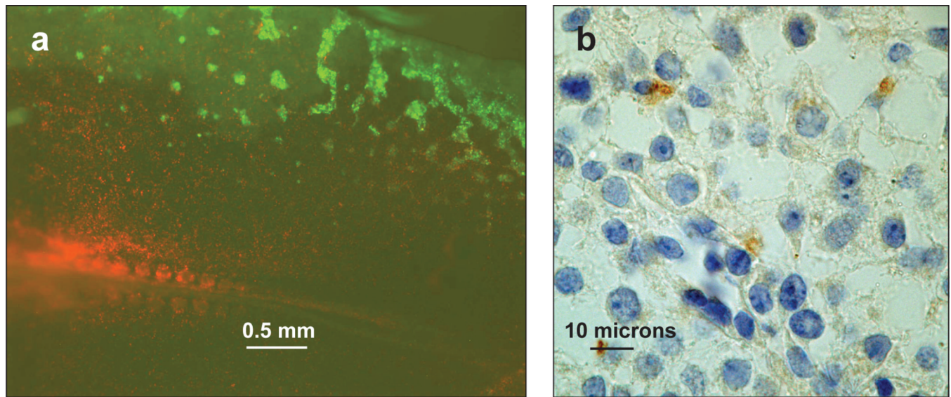
Figure 4. Transgenic analysis implicates involvement of Hox CNE HA14E1 in extraembryonic activities in the chick and mouse
