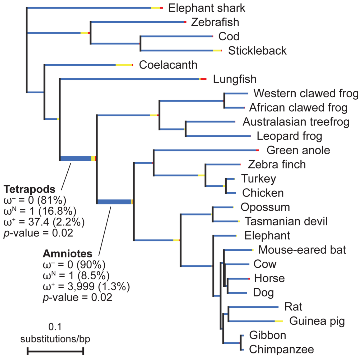
Figure 3. Phylogeny of CPS1 coding sequences used to determine positive selection within the urea cycle
