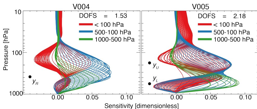
Fig. 1. Typical averaging kernel matrices for TES methane retrievals over the tropical ocean: V004 (left) and V005 (right). Data are from the same target on 7 November 2009 at 1.1° S and 166.9° W. Lines are the individual rows of the averaging kernel matrix and represent the sensitivities of retrieved methane at given pressure levels to methane concentrations throughout the atmospheric column. Black circles indicate the pressure levels used for comparison to the HIPPO aircraft observations.
