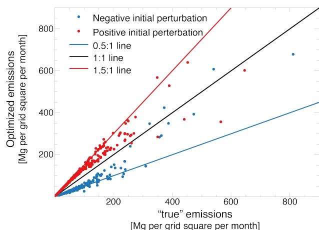
Fig. 9. Scatterplot of optimized vs. “true” methane emissions for individual 4^{\circ} \times 5^{\circ} grid squares. Blue and red points show emissions with negative and positive a priori perturbations, respectively. The a priori perturbations correspond to the blue and red lines.
