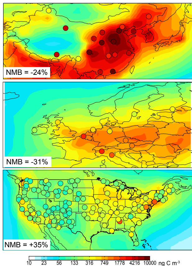
Fig. 3. Annual mean surface air concentrations of BC aerosol in China, Europe, and the US. Model results for 2008 (solid contours) are compared to observations (circles). Observations are from Zhang et al. (2008a) in China for 2006, from the EMEP network in Europe for 2002–2003 ( http://tarantula.nilu.no/projects/ccc/emepdata.html ), and from the IMPROVE network in the US for 2008 ( http://vista.cira.colostate.edu/improve/Data-IMPROVE/AsciiData.aspx ). Normalized mean bias (NMB) statistics for each region are shown inset.
