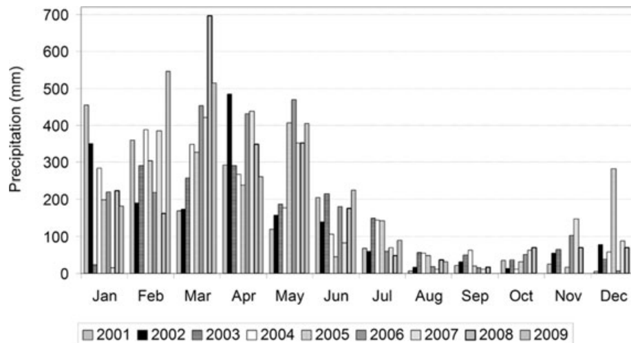
Fig. 7. Precipitation by month for each year from http://hyd88.eng.uci.edu/hydis-unesco/ using four squares: (a) latitude from 2^{\circ} to -4^{\circ} and longitude from -55^{\circ} to -32^{\circ} ; (b) latitude from -4^{\circ} to -6^{\circ} and longitude from -50^{\circ} to -32^{\circ} ; (c) latitude from -6^{\circ} to -8^{\circ} and longitude from -45^{\circ} to -32^{\circ} and (d) latitude from -8^{\circ} to -10^{\circ} and longitude from -40^{\circ} to -32^{\circ} .
