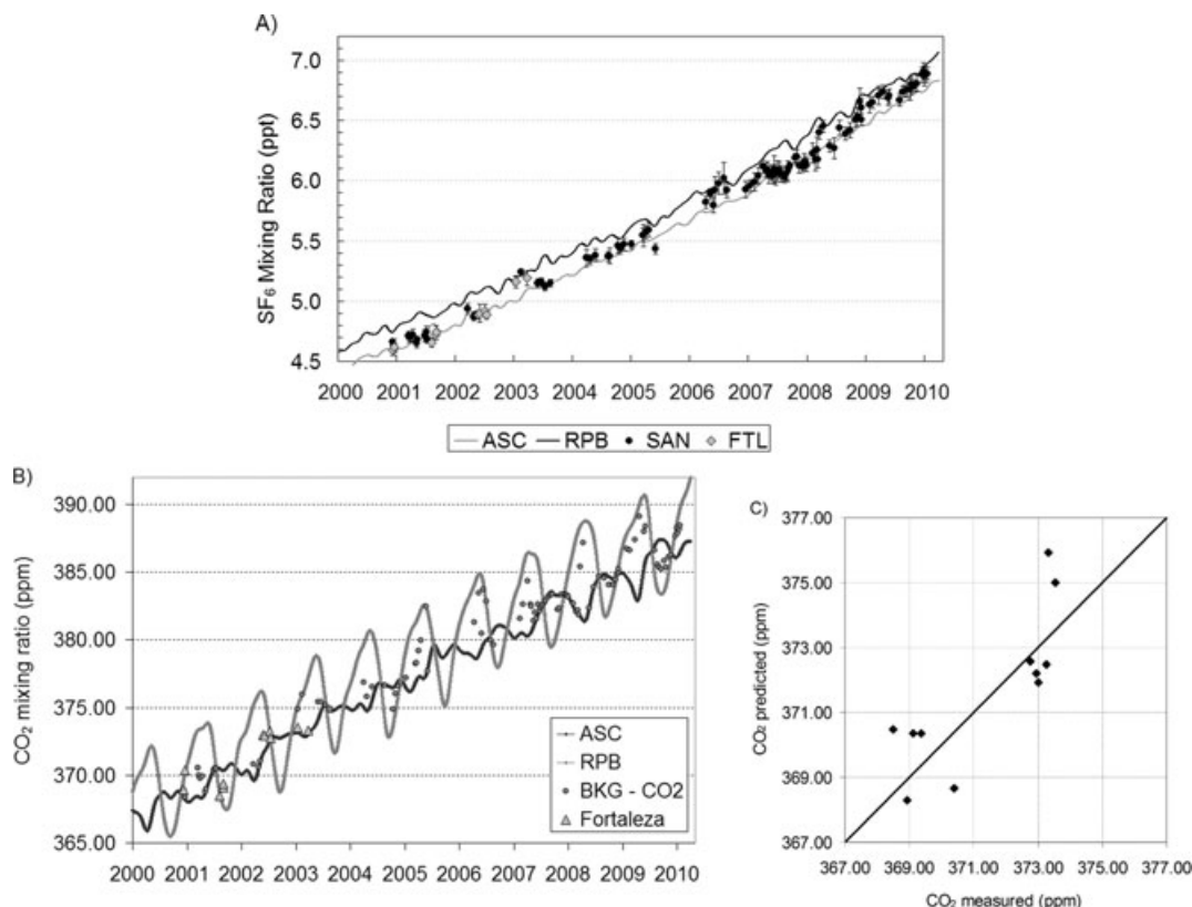
Fig. 3. (a) SF 6 time series from Ascension Island ASC (grey line), Barbados Island RBP (black line), SAN average vertical profile (black circle) and Fortaleza average vertical profile (grey lozenge). (b) CO 2 time series from Ascension Island ASC (grey line), Barbados Island RBP (black line) and CO 2 BKG calculated by eq. 2 (black circle) and Fortaleza average vertical profile (grey diamond). (c) Correlation between CO 2 background predicted by SF 6 method and CO 2 measured in Fortaleza profile, where the correlation coefficient ( r^2 ) is 0.7.
