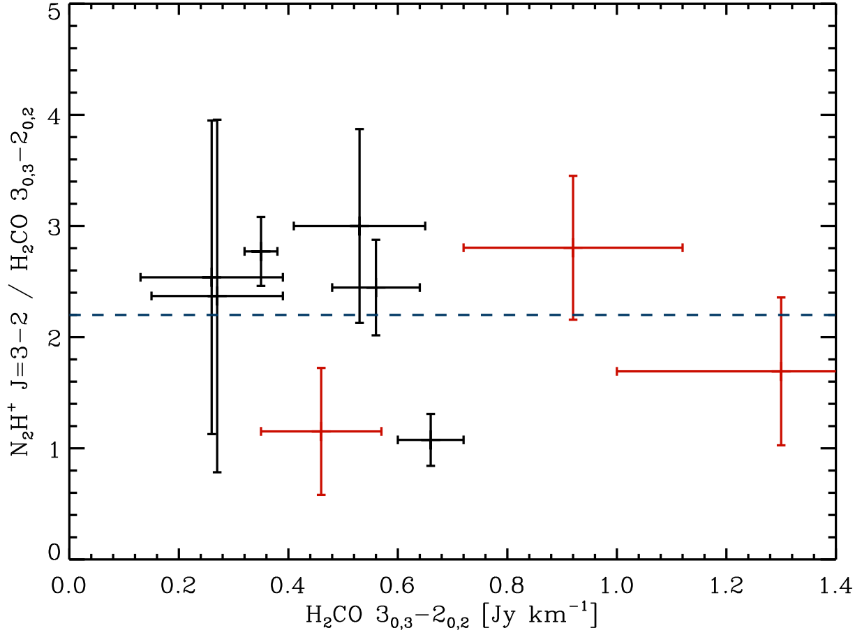
Fig. 10.— The \text{N}_2\text{H}^+/\text{H}_2\text{CO} ratio, demonstrating that it is almost constant, as would be expected from the strong correlation between the normalized fluxes.
