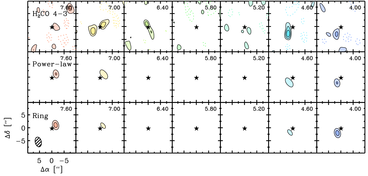
Fig. 5.— As Fig. 4 but for the H 2 CO 4 1,4 – 3 1,3 line.
