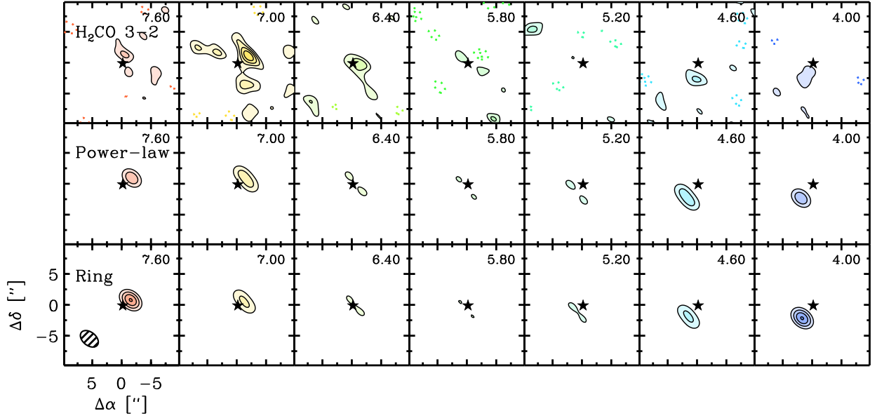
Fig. 4.— Observed and simulated channel maps for \text{H}_2\text{CO } 3_{1,2} - 2_{1,1} toward HD 163296, using the best-fit power-law ( p=2 ) and ring model. Both models fit the data within the uncertainties. The first contour is 2\sigma and each following contour step is 1\sigma . The channel velocity in \text{km s}^{-1} is in the upper right corner of each panel and the synthesized beam is displayed in the lower left panel.
