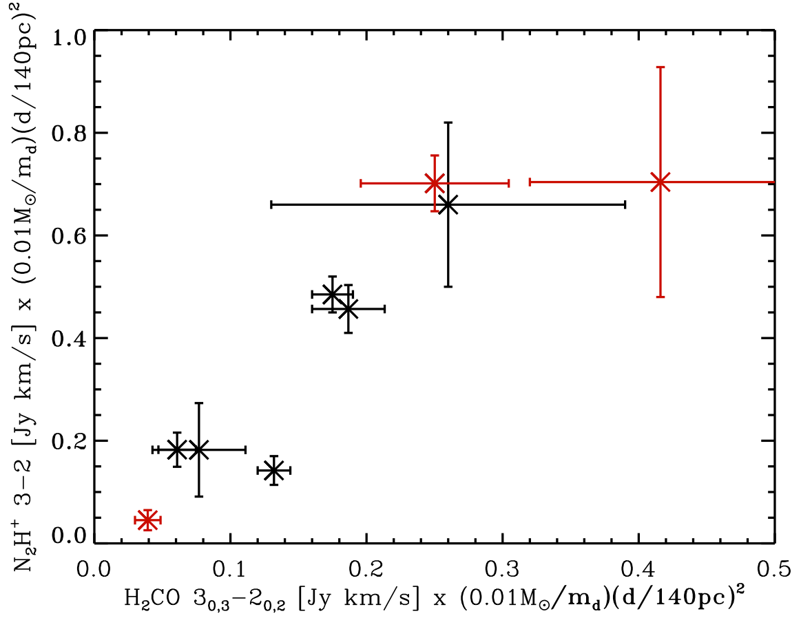
Fig. 9.— Correlation of \text{N}_2\text{H}^+ 3-2 ( E_u = 27 K) and \text{H}_2\text{CO } 3_{0,3} - 2_{0,2} ( E_u = 21 K) emission normalized to disk mass (based on dust modeling) and source distance. The red symbols mark disks where the \text{H}_2\text{CO } 3_{0,3} - 2_{0,2} flux has been calculated based on the flux from other \text{H}_2\text{CO} transitions.
