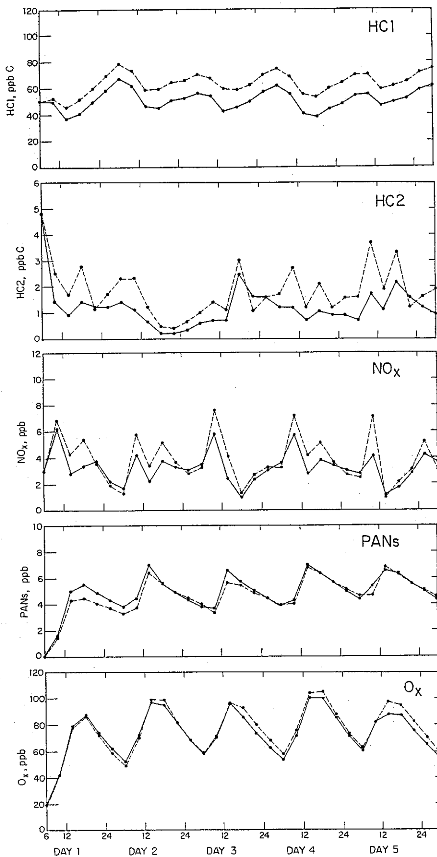
Fig 4. Time evolution of tracer concentrations in the 5-day test simulation. Results from the LIV simulation (solid line) and from the CONTROL simulation (dashed line) are compared.
