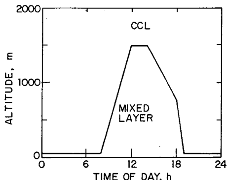
Fig. 2. Height of the mixed layer as a function of time of day.
