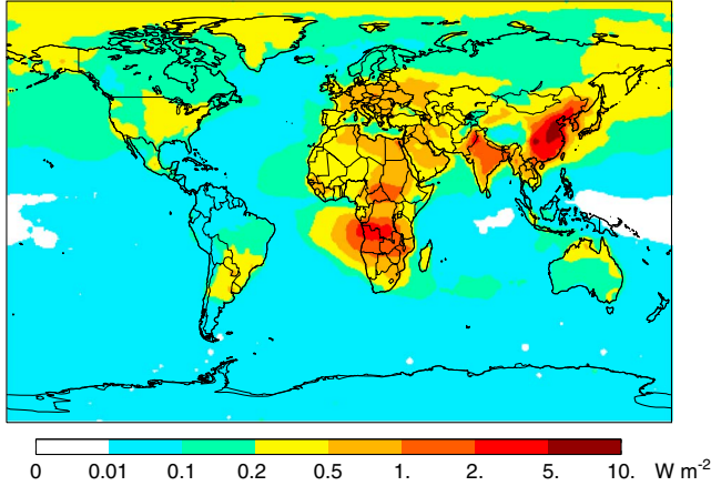
Figure 11. Global annual mean distribution of BC direct radiative forcing (DRF) at the top of the atmosphere (TOA). The radiative transfer model of Wang et al. [2008, 2013] is applied to the 3-D distribution of BC mass concentrations from GEOS-Chem.
