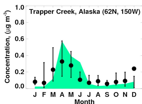
Figure 7. Seasonal variation of fine mode dust aerosol ( <2.5 \mu\text{m} diameter) concentrations at Trapper Creek, Alaska, in 2008. Observations for 2008 are shown as black symbols, and vertical bars show the interannual standard deviation for the period 2001–2009. The observations are further described in Table 1. Model values are shown as green contours.
