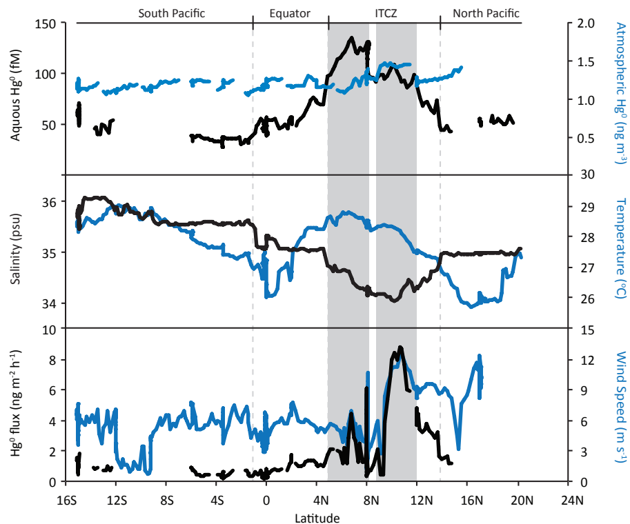
Figure 1. Latitudinal variability in measured atmospheric and seawater Hg 0 concentrations, associated evasion, and environmental properties on the METZYME cruise between 1-24 October, 2011. Oceanographic regimes for October 2011 are shown; shaded areas denote statistically different regions for Hg 0 concentrations within the oceanic regime reflecting the ITCZ.
