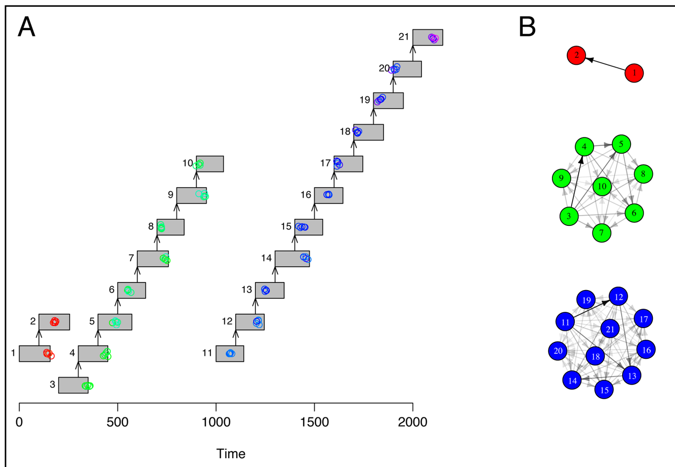
Fig 6. Evolutionary dynamics and estimated routes of infection on a disconnected transmission tree. We simulated evolutionary dynamics on top of a pre-specified transmission tree, in which three cases are imported to the community under observation. (A) Genomes are represented by colored circles, colored according to genetic distance from the first sampled genome in individual 1; red denotes an identical genotype, while colors closer to the blue end of the spectrum denote an increasing genetic distance from this reference genome. The expected genetic distance between imported cases was 12 SNPs. (B) Estimated routes of infection. We assumed that recovery times were not observed, such that any previously infected host could be the source of infection at the time of transmission. Routes with posterior probability < 0.05 are not shown. This network diagram was plotted using the igraph package [32].
