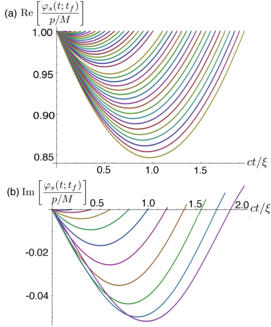
FIG. 5. (Color online) (a) Real part of the (rescaled) solution of saddle-point equation (54) plotted for m_r = 75.0 , \sqrt{n_0}\xi a_{IB,\sigma} = 0.25 , p/Mc = 0.6 ; we obtained a family of trajectories parametrized by t_f , the total propagation time for which the amplitude (52) was required. Each individual trajectory is a time-evolving function of t < t_f , and can be interpreted (after rescaling) as the time-dependent momentum of the impurity. Note the symmetry of the saddle-point trajectories around t = t_f/2 , which arises because they optimize Eq. (52), the amplitude for a time-evolving state to return to its initial value. This is in contrast to the time-dependent mean-field solution which simply propagates forward to the steady state at time t_f (cf. Fig. 6). (b) Imaginary part of the saddle-point trajectories are shown for the same parameters. The imaginary part shares the symmetry property of the real part, but is typically smaller in magnitude. While it does not lend itself to direct interpretation as the physical momentum of the impurity, it is necessary to properly optimize the propagation amplitude when expressed as a path integral equation (53).
