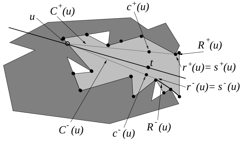
Figure 6: R^-(u) , R^+(u) , r^-(u) , r^+(u) , s^-(u) and s^+(u) .
