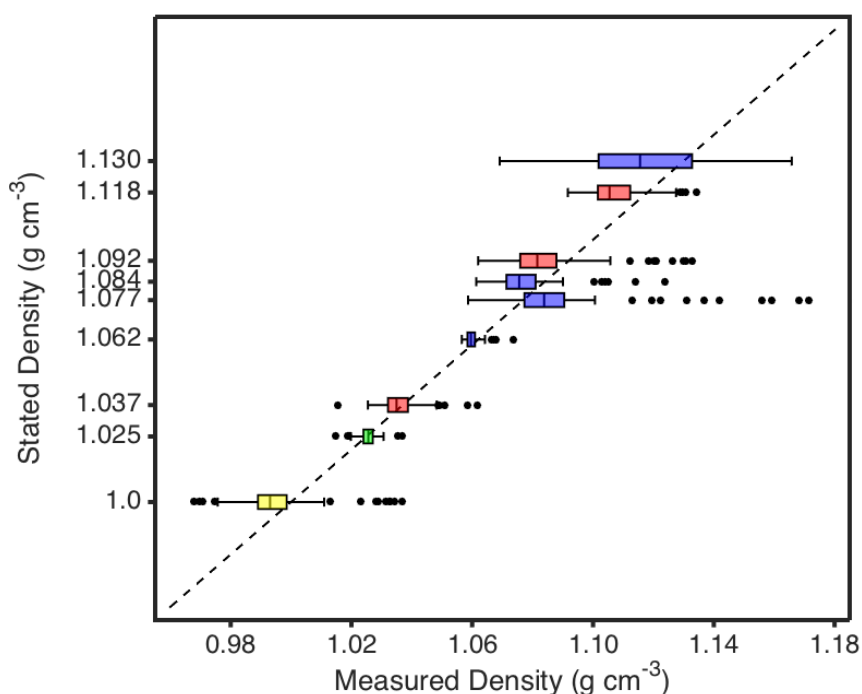
Figure 2. Box plots showing the distribution in density for 200–300 \mu\text{m} diameter polymer microsphere purchased from CoSpheric LLC. In these box plots and all others in this paper, the box extends from the 25 th percentile to the 75 th percentile and with the central line marking the median density. The whiskers extend from the end of the box a maximum of 1.5 times the change in density from the 25 th to 75 th percentile; whiskers do not extend beyond the most extremal datum. Additional points represent outliers. The colors of the boxes represent the color of the beads as purchased. Mean densities and distributions in density were measured using MagLev ( n = 78\text{-}191 ). The dotted line represents a 1:1 relationship between the density stated by the manufacturer and the density as measured in our experiments.
