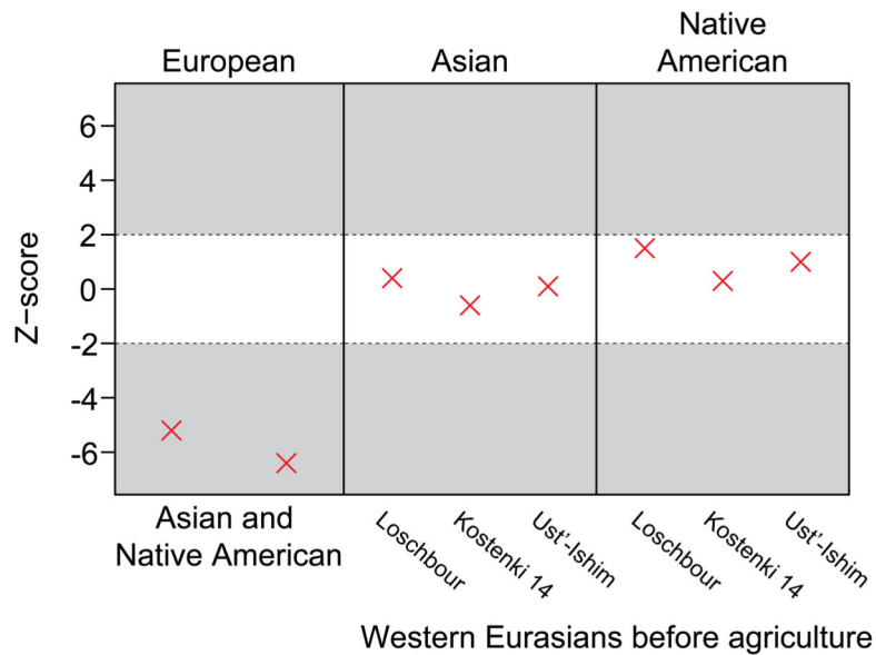
Figure 1. Allele sharing between the Oase 1 individual and other genomes Each point indicates the extent to which the Oase 1 genome shares alleles with one or the other of a pair of genomes from different populations indicated above and below (see Extended Data Table 1 for numbers). Z-scores larger and smaller than |2| indicate an excess of allele sharing (grey).
