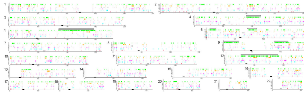
Figure 2. Spatial distribution of alleles matching Neanderthals in modern humans
