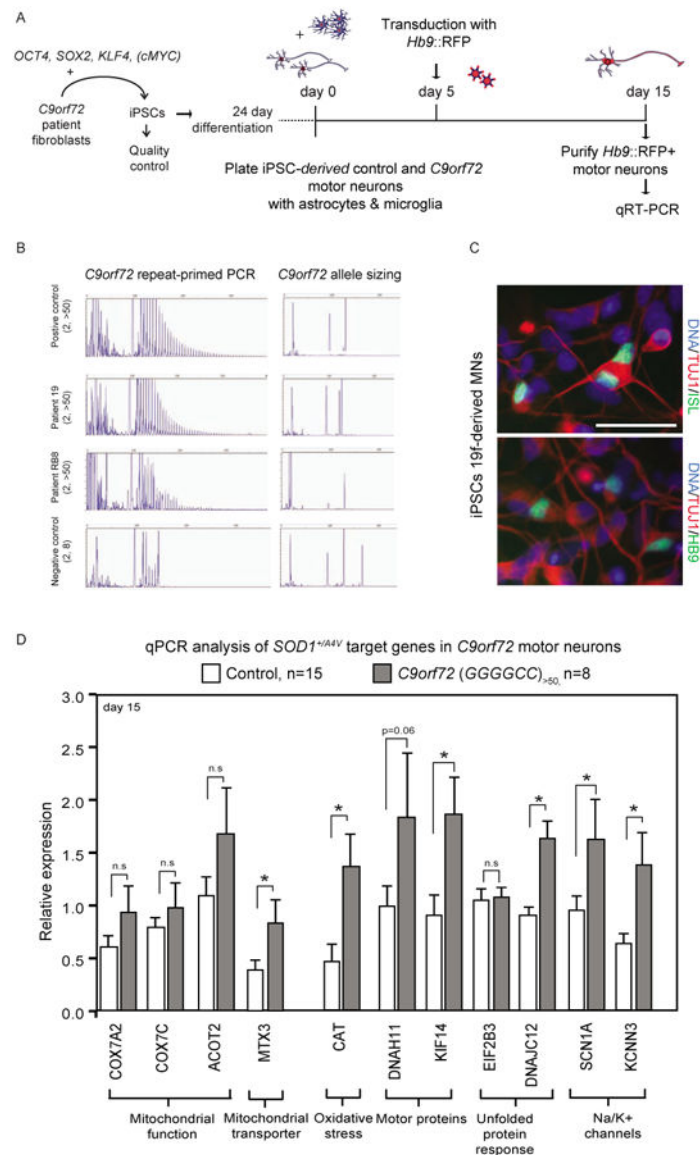
Figure 7. Transcriptional Changes Detected in SOD1 +/A4V Motor Neurons are Partially Conserved in Motor Neurons With C9orf72 Expansions
