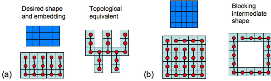
Figure 2: MakeTreeGrammar provides grammars that preserve topology but not geometry. Simply embedding a tree in a 2D shape can result in two different kinds of problems (a) the generated shape is a topological equivalent of the desired shape (b) the topologically-valid, partially-generated, shape blocks physical access to modules.
