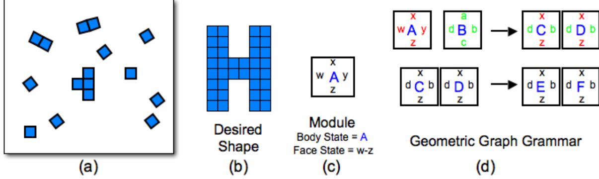
Figure 1: Abstract Self-Assembly Framework: (a) We assume square modules moving in a 2D space (b) The desired goal is specified as a 2D grid shape (c) Each module has body and face states (d) Modules interact according to geometric grammar rules. The top rule shows that if two modules with body states A and B meet along the y and d faces respectively (LHS), they can attach together and as a result of their attachment both their body and face states change in an orientation specific manner (RHS). It is also possible to have rules that operate on attached modules and only change the body/face states.
