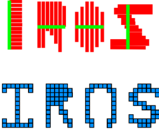
Figure 9: Examples of the structure classes for which MakeGridGrammar and CollectiveAssembly are provably correct. MakeGridGrammar (top): structures that can be drawn as straight backbones (green) plus orthogonal straight side chains (red). CollectiveAssembly (bottom): more general structures without internal holes.
