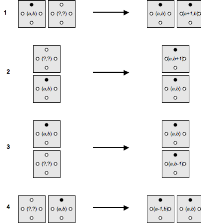
Figure 5: Four rules by which a new module becomes attached to an existing one at coordinates (a,b) , and acquires coordinates and orientation to match the rest of the assembly. Coordinates are given in the center of the module; orientation is shown by having the north face marked with a black dot.
