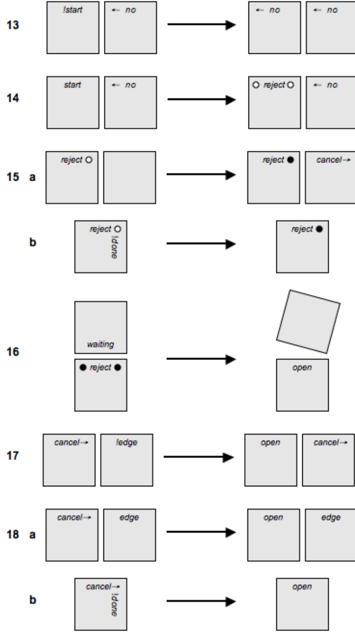
Figure 12: Modified rules for attachment when multiple modules may be present to try to bind at the same time to the same open row: part III.
