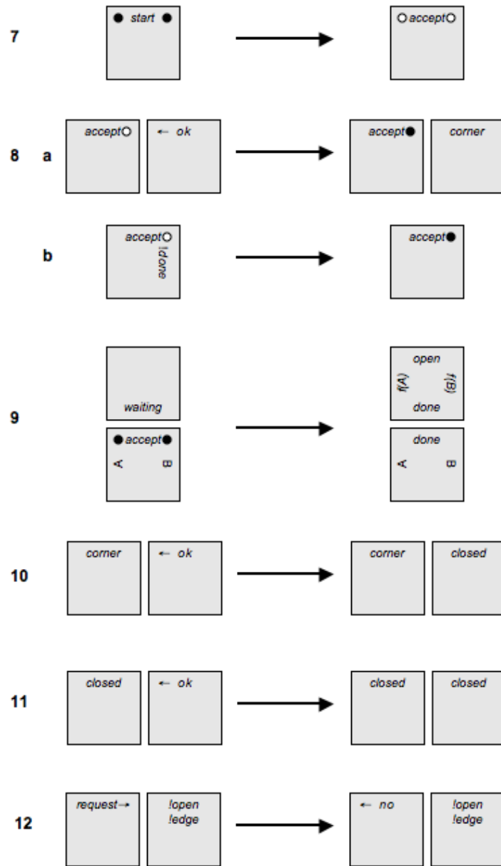
Figure 11: Modified rules for attachment when multiple modules may be present to try to bind at the same time to the same open row: part II.
