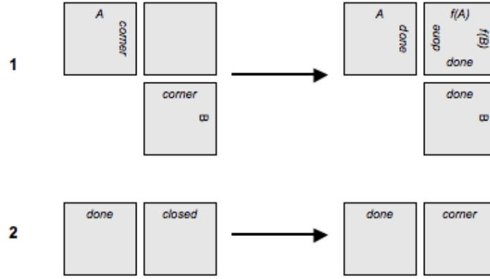
Figure 7: Rules for attachment in rows where modules have already been attached. In such rows, attachment is permitted only at corner sites. (1) The attachment can be completed immediately, without the need to propagate information down the row. The states of the other faces of the newly added module are set based on the analogous faces of the previously existing modules A and B , with the function f defined in the text. (2) Once attachment is completed, the next adjacent site (if any) is unlocked by setting it to corner .
