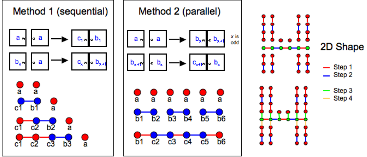
Figure 4: Best-case parallelism: Two different grammars for a chain that create two different self-assembly processes. Method 1 forces the chain to form sequentially, while method 2 allows the chain to assemble its part in parallel. By exploiting parallel chain formation, it is possible to generate any 2D-backbone shape in just 4 steps.
