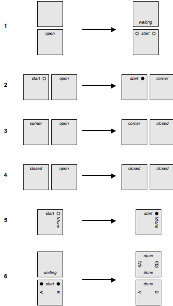
Figure 6: Rules for attachment in rows where no modules have yet been attached. In these pictures, any states not explicitly specified are to be treated as wildcards and may be any state. (The exception is the completely unmarked module, which represents the new one potentially becoming attached.) All rules shown as non-symmetric should be understood to apply in reflection as well.
