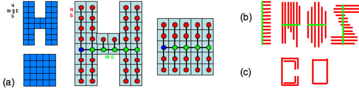
Figure 3: MakeGridGrammar: (a) Given a desired shape, the embedding creates a tree with a linear chain backbone and sidechains (b) Example of shapes in the 2D-backbone shape class (c) Examples of shapes that cannot be formed.
