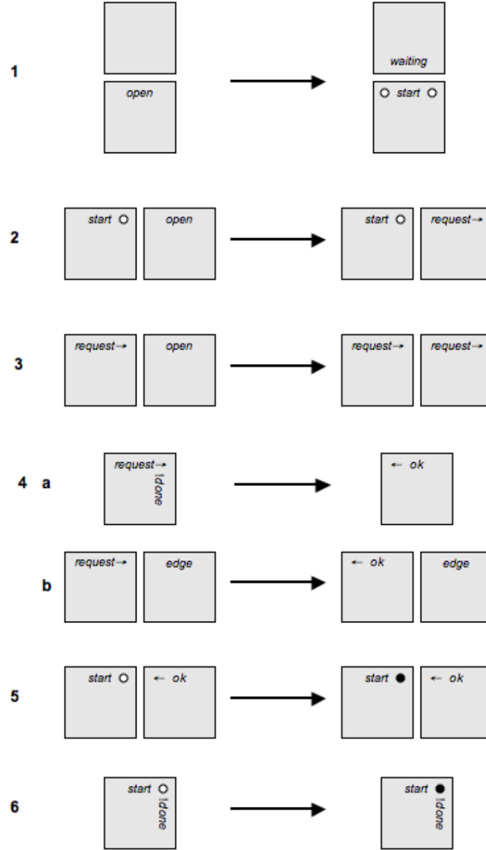
Figure 10: Modified rules for attachment when multiple modules may be present to try to bind at the same time to the same open row: part I.
