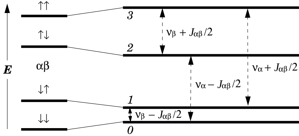
Figure 1. The four energy levels associated with two spins \alpha and \beta , whose resonance frequencies are \nu_\alpha and \nu_\beta Hertz. The energy levels when there is no coupling between the spins are shown on the left, and those with a coupling of J_{\alpha\beta} Hertz on the right. The allowed transitions between the energy levels are indicated with two-headed dashed arrows.
