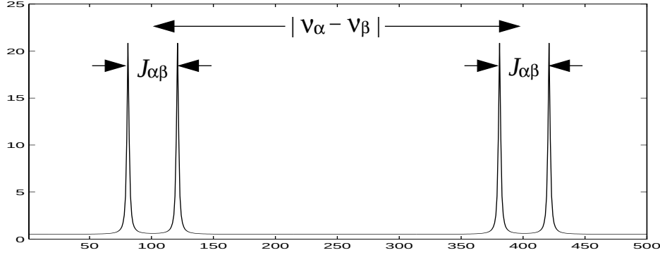
Figure 2. The simulated NMR spectrum of a two-spin system, with \nu_\alpha = 100 , \nu_\beta = 400 and J_{\alpha\beta} = 40 Hertz. From left to right, the four peaks in this spectrum correspond to the transitions 0 \leftrightarrow 1 , 2 \leftrightarrow 3 , 0 \leftrightarrow 2 and 1 \leftrightarrow 3 indicated in Fig. 1 (be forewarned, however, that NMR spectroscopists traditionally plot their spectra with frequency increasing from right to left). In practice, this spectrum would be obtained by applying a nonselective \pi/2 pulse to the equilibrium state and Fourier transforming the resulting signal. The peak intensities are proportional to the population differences between pairs of states, and their widths to the inverse decoherence time (known as T_2 in NMR).
